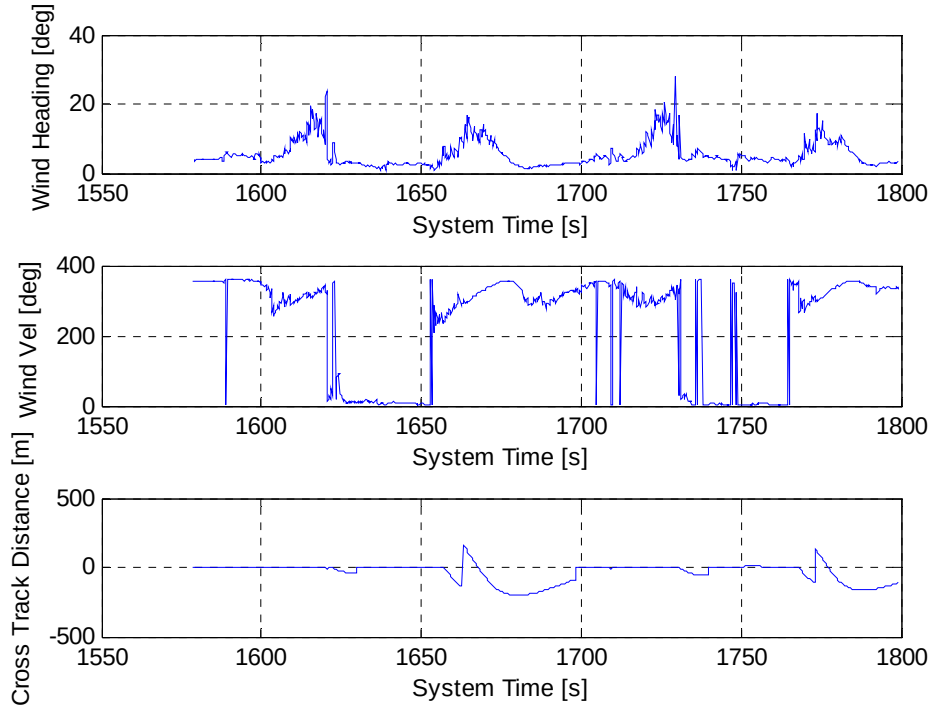
Figure 100. Various Parameters for the Race Track Pattern at 30 m/s, Wind5 m/s, & TC=250
