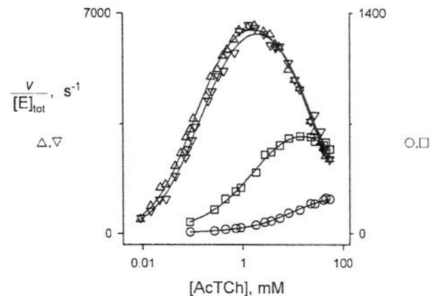
FIG. 2. Dependence of normalized hydrolysis rates on the acetylthiocholine concentration for H287C AChEs modified by MTS reagents. Hydrolysis rates v were measured at the indicated acetylthiocholine concentrations as outlined under "Experimental Procedures." Values were obtained for unmodified H287C AChE ( \Delta ) and H287C AChEs modified with MTS reagents II ( \nabla ), IV ( \square ), and V ( \circ ) and isolated as shown in Fig. 1. The line for unmodified AChE was calculated by fitting the data to Equation 1. Lines for the modified AChEs were calculated by fitting the data to Equation 2. Each data set was normalized by dividing the measured activity by the concentration of total enzyme present in the assay: unmodified H287C AChE ( \Delta ), 87 pM; II ( \nabla ), 61 pM; IV ( \square ), 510 pM; and V ( \circ ), 980 pM. The calculated percentages of modified enzyme in the preparations were 31 \pm 20 , 98 \pm 1 , and 99 \pm 1 , for II, IV, and V, respectively.
