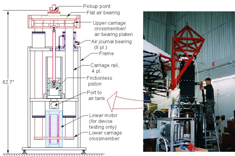
Figure 10 7000-lb truss testbed structure floated on three floor-standing zero-G suspension devices. Horizontal motion at each support point is allowed by a flat air bearing running on the ceramic upper crossmember platen of the device.
