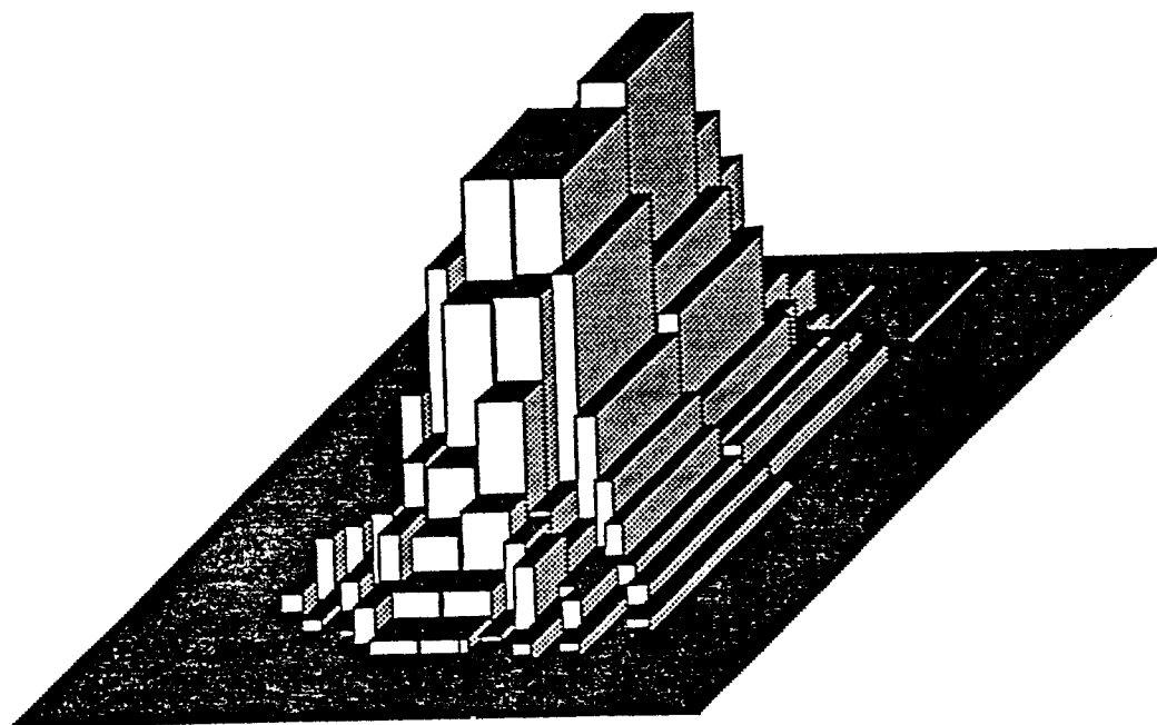
Figure 4.2.19. Semigridded histogram (density as in Figure 4.2.15, sample size = 2000).
