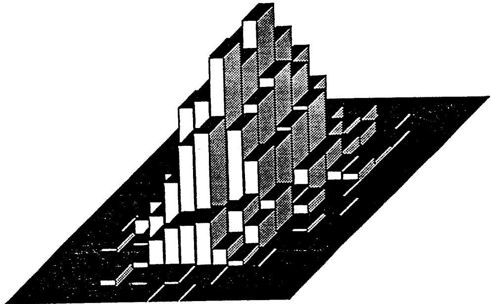
Figure 4.2.16. Regular histogram (density as in Figure 4.2.15, sample size = 2000).
