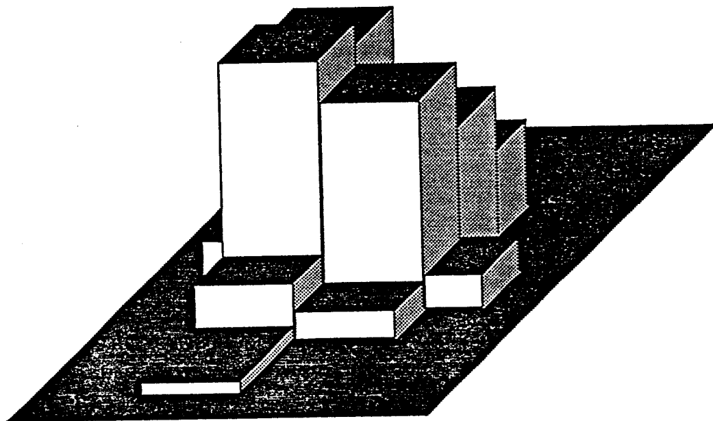
Figure 4.2.1. Grid histogram based upon a sample size of 50 from the bivariate normal density 3.4.1 with p = .5 , \rho_1 = \rho_2 = 0 , \sigma_1 = \sigma_2 = \sigma_3 = \sigma_4 = 1 , \mu_1 = -1 , \mu_2 = 0 , \mu_3 = 1 , \mu_4 = 0 .
