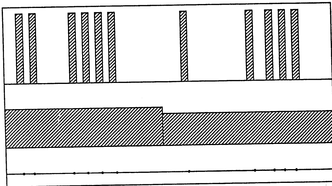
Figure 1.1. Above: example of histogram in which h is too small so that \hat{f} is too rough (variance is large and bias is small). Below: example of histogram in which h is too large so that \hat{f} is too smooth (variance is small and bias is large).
