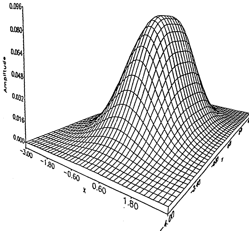
Figure 4.2.15. Bivariate normal density 3.4.1 with p = .5 , \rho_1 = \rho_2 = 0 , \sigma_1 = \sigma_2 = \sigma_3 = \sigma_4 = 1 , \mu_1 = 0 , \mu_2 = -1 , \mu_3 = 0 , \mu_4 = 1 .
