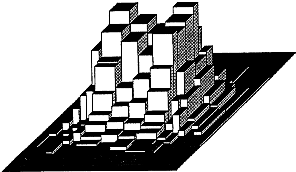
Figure 4.2.29. Semigridded histogram (density as in Figure 4.2.25, sample size = 2000).
