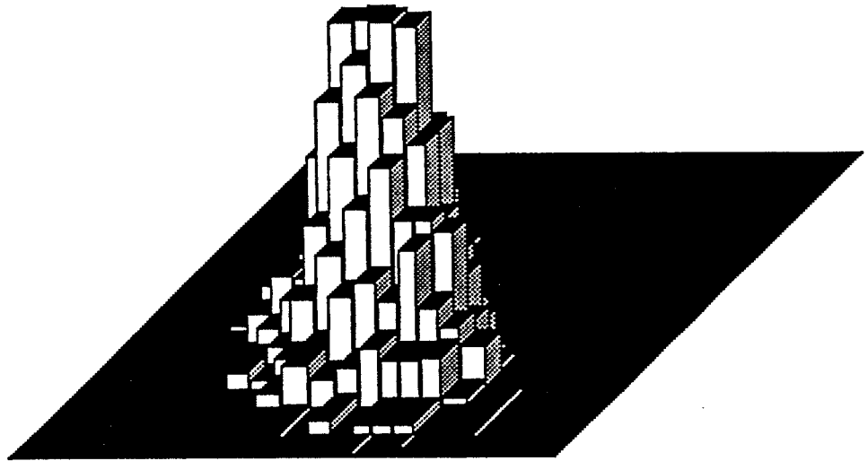
Figure 4.2.46. Grid histogram (density as in Figure 4.2.43, sample size = 2000).
