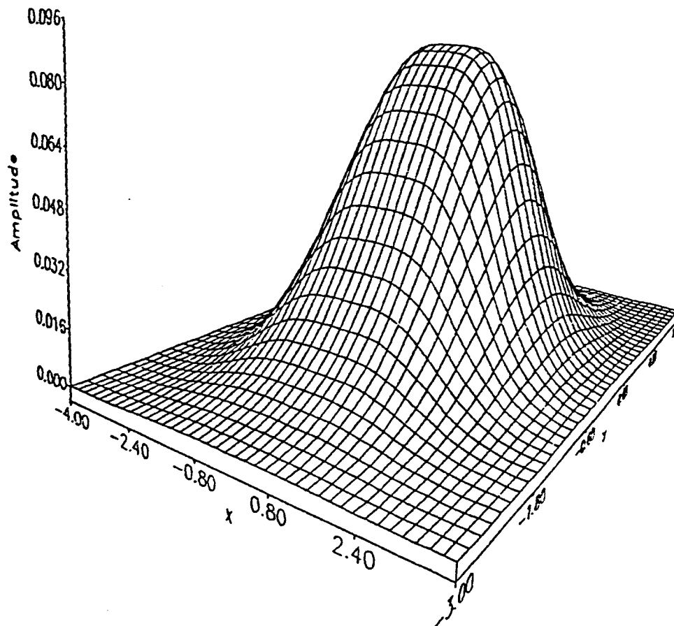
Figure 4.2.10. Bivariate normal density 3.4.1 with p = .5 , \rho_1 = \rho_2 = 0 , \sigma_1 = \sigma_2 = \sigma_3 = \sigma_4 = 1 , \mu_1 = -1 , \mu_2 = 0 , \mu_3 = 1 , \mu_4 = 0 .
