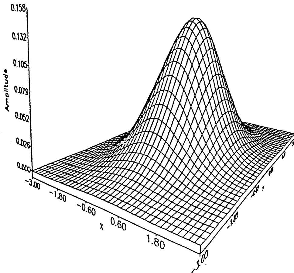
Figure 4.2.5. Bivariate normal density 3.4.1 with p = 1 , \rho_1 = \rho_2 = 0 , \sigma_1 = \sigma_2 = \sigma_3 = \sigma_4 = 1 , \mu_1 = \mu_2 = \mu_3 = \mu_4 = 0 .
