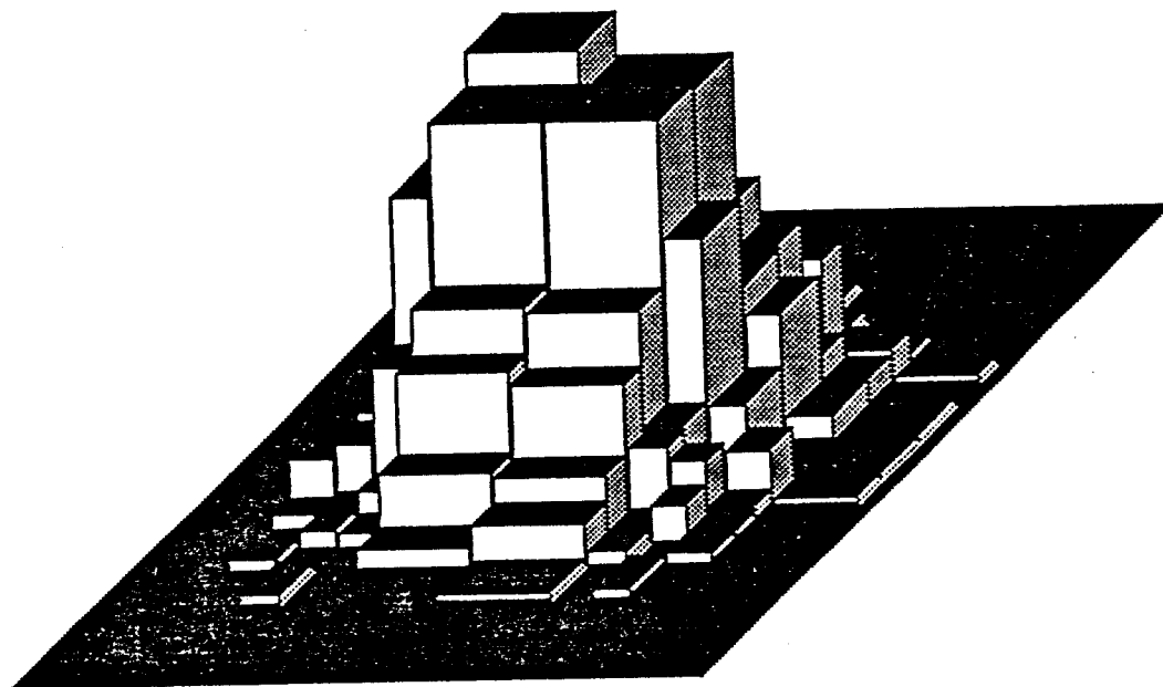
Figure 4.2.3. Grid histogram based upon a sample size of 1000 (parameters same as in Figure 4.2.1).
