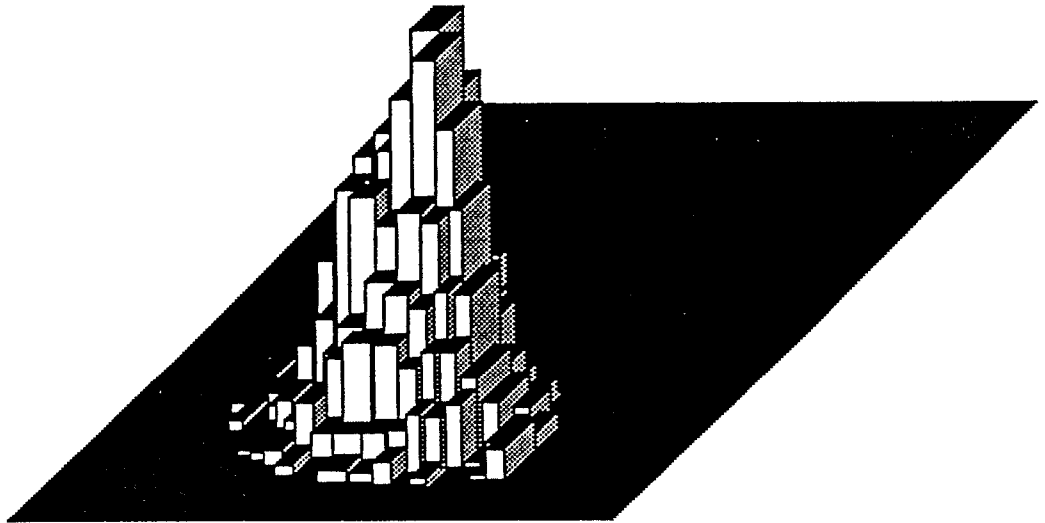
Figure 4.2.47. Semigridded histogram (density as in Figure 4.2.43, sample size = 2000).
