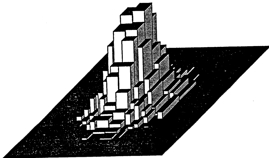
Figure 4.2.9. Semigridded histogram (density as in Figure 4.2.5, sample size = 2000).
