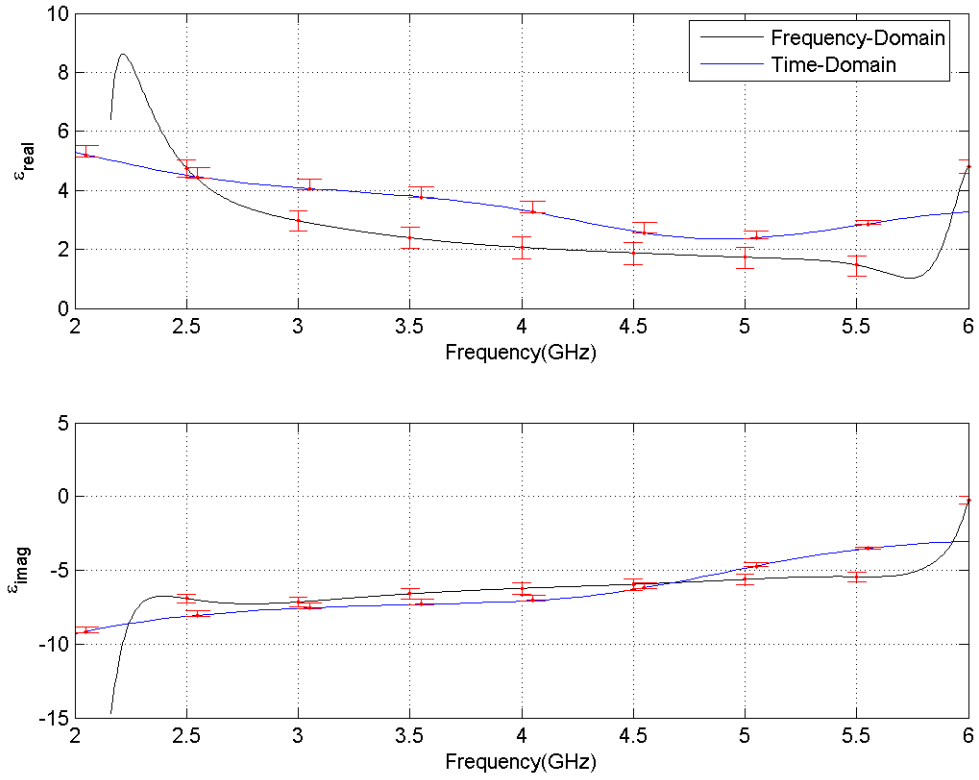
Figure A.5: Complex permittivity of 125 mil ERAM sample measured with the focus arch free-space system from 2-6 GHz for the frequency-domain method and direct time-domain method.
