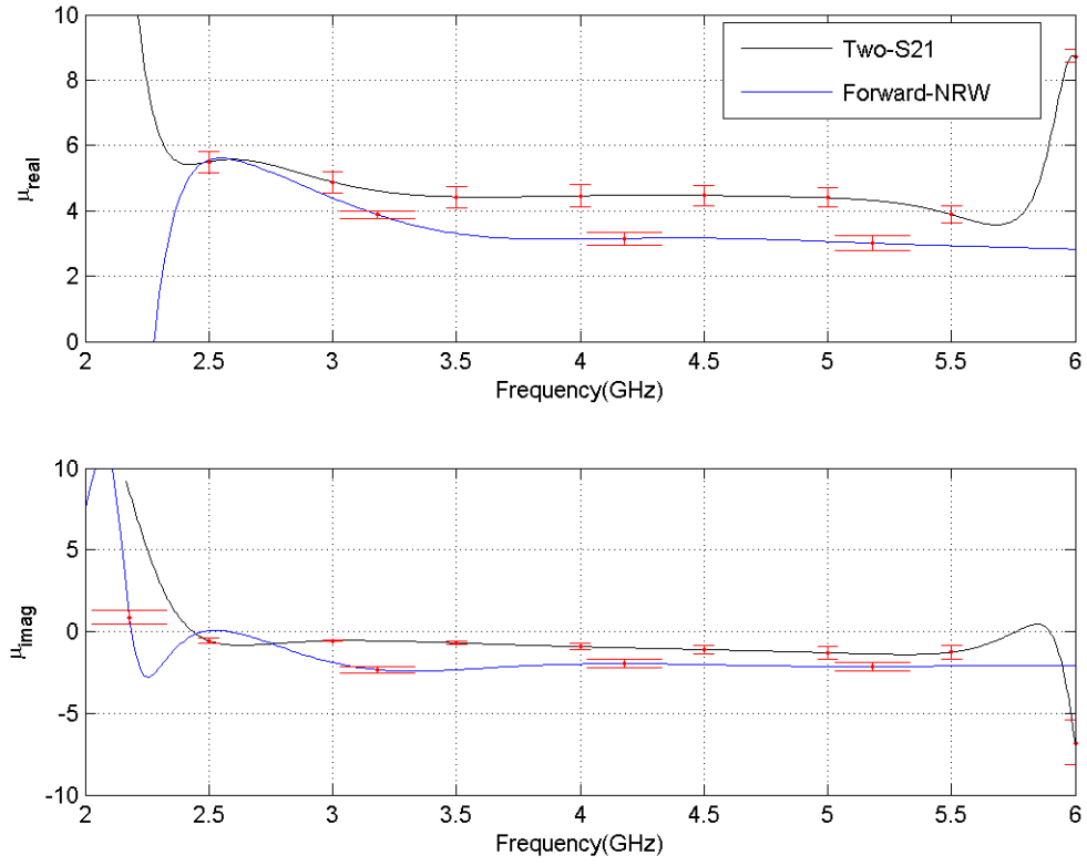
Figure 4.7: Permeability of MRAM sample measured with the focus arch free-space system from 2-6 GHz for the forward NRW and two transmission method.
