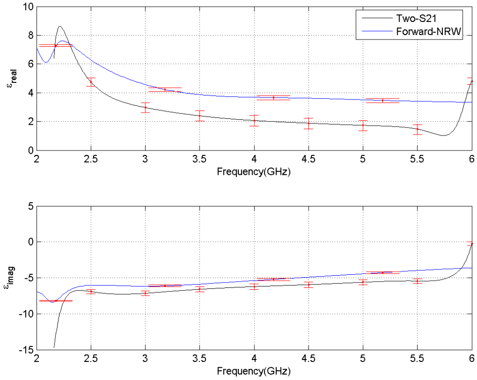
Figure A.3: Complex permittivity of 125 mil ERAM sample measured with the focus arch free-space system from 2-6 GHz for the forward NRW and two transmission method.
