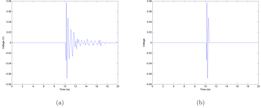
Figure 3.10: (a) Raw measured forward voltage measurement V(t)_{21}^{exp, meas1} using oscilloscope prior to calibration of a single-layer sample in time-domain focus arch system. (b) Time gated forward voltage measurement V(t)_{21}^{exp, meas1} prior to calibration of a single-layer sample in time-domain focus arch system.
