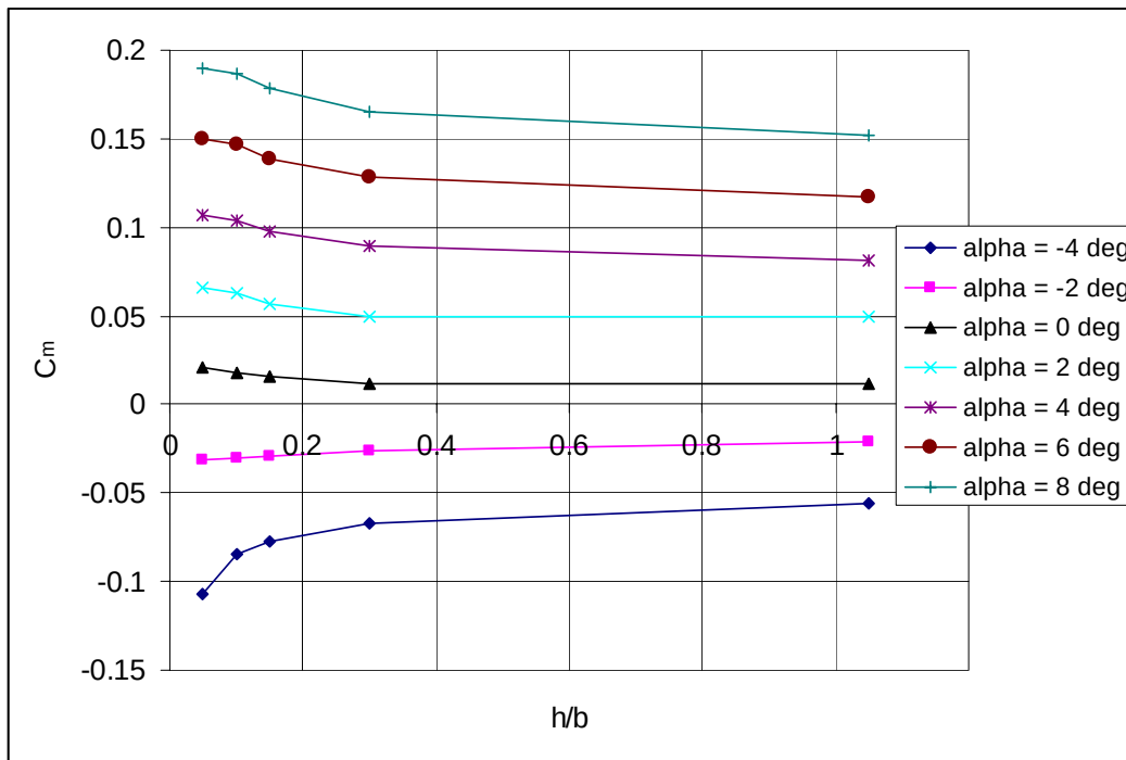
Figure 105: Ground Effect, C_m vs. (h/b) , Flaps +10^\circ , 100 mph
