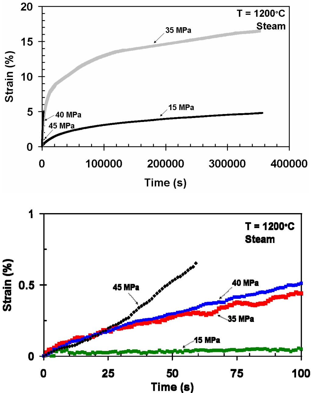
Figure 34. Creep-strain vs. time in 100% steam at 1200°C.
