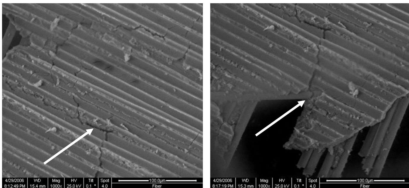
Figure 61. SEM micrographs depicting cracks propagating through matrix.
