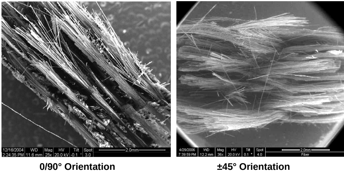
Figure 66. SEM micrographs depicting fracture surfaces of N720/A specimens with 0/90^\circ and \pm 45^\circ fiber orientations.
