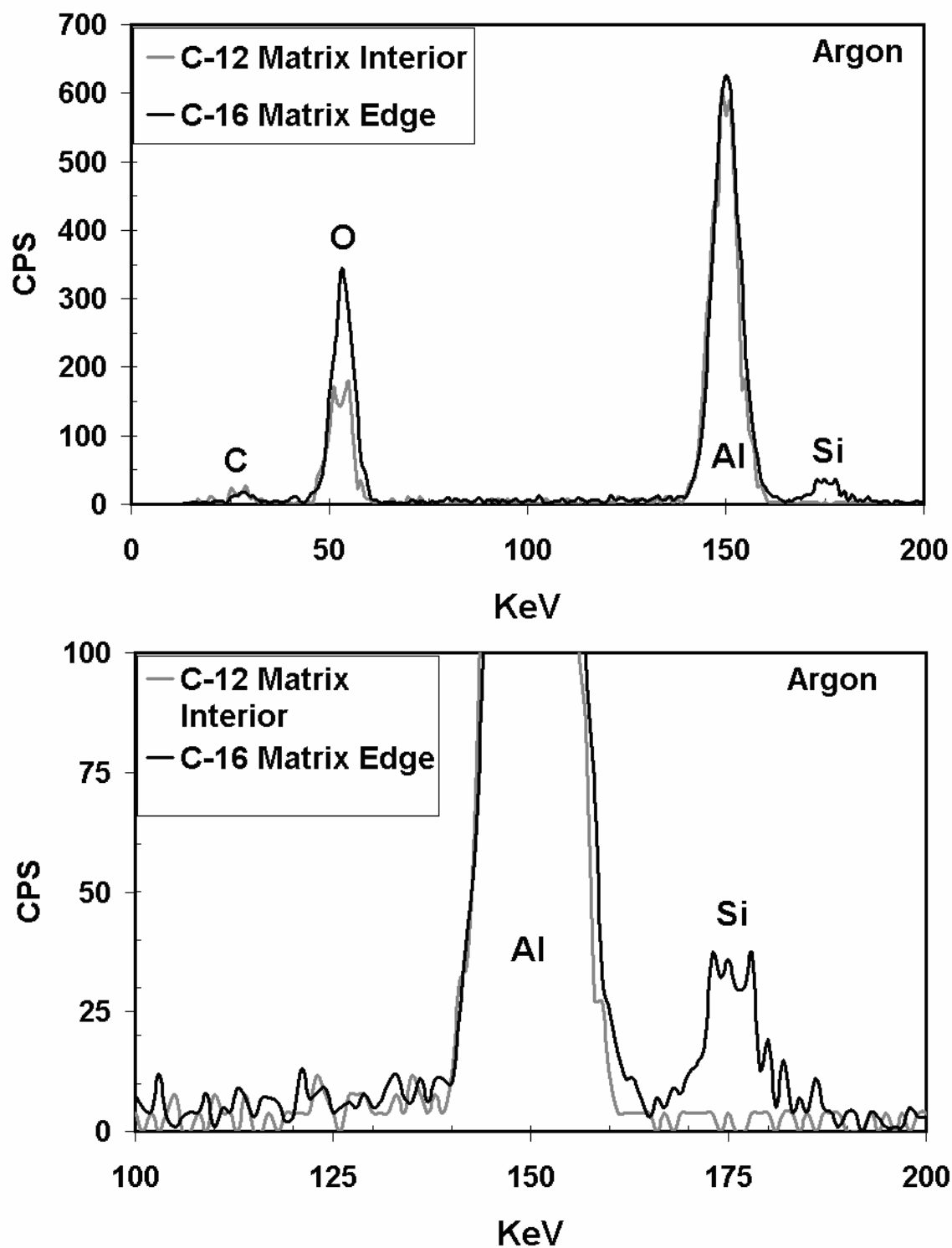
Figure 74. EDS spectra of the matrix interior compared to the spectra of the matrix edge in the specimens tested in 100% argon.
