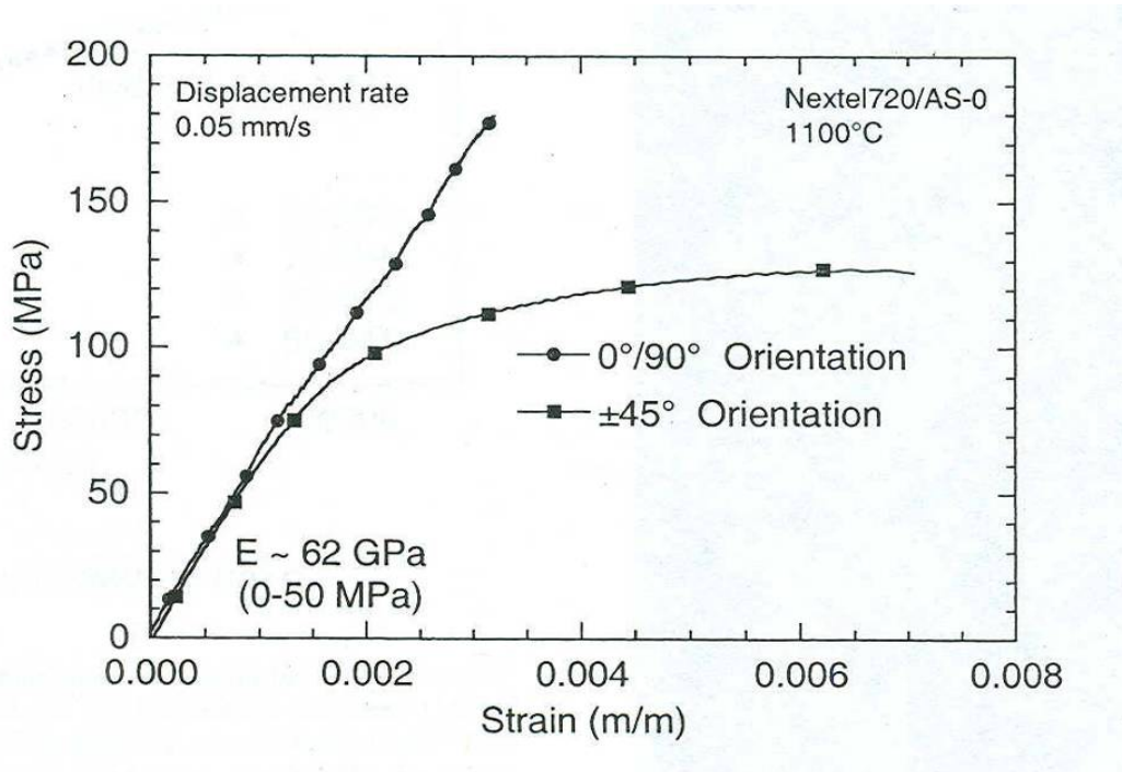
Figure 8. Stress vs. strain of N720/AS in 0/90° and \pm 45^\circ orientation at 1100°C. N720/AS with the \pm 45^\circ fiber orientation produced much lower ultimate tensile strength (UTS) compared to the UTS obtained for the 0/90° fiber orientation. [8:457].
