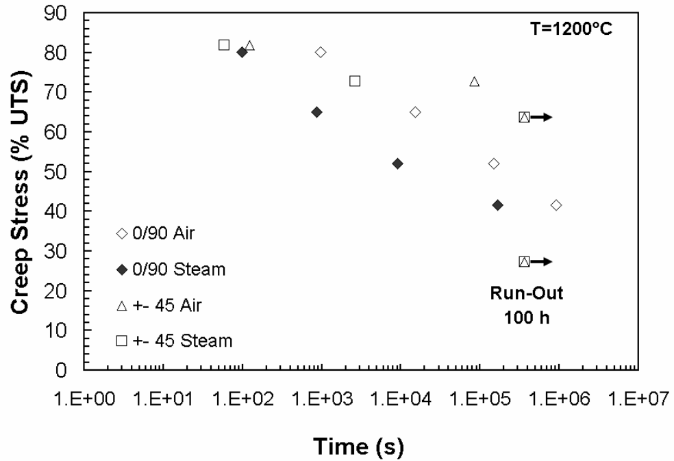
Figure 42. Creep-stress vs. time to failure for N720/A with 0/90° and \pm 45^\circ fiber orientations at 1200°C in air and in steam environments.
