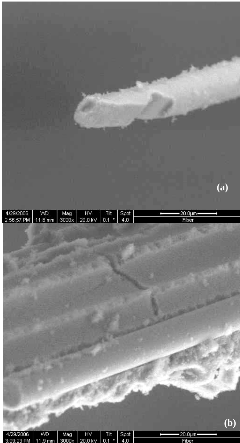
Figure 101. Micrograph of Nextel TM 720/alumina CMC specimen C-17 tested in creep at 45 MPa at 1200°C in 100% argon environment: (a) individual fiber with irregular fracture pattern, (b) crack propagating between matrix separating fibers.
