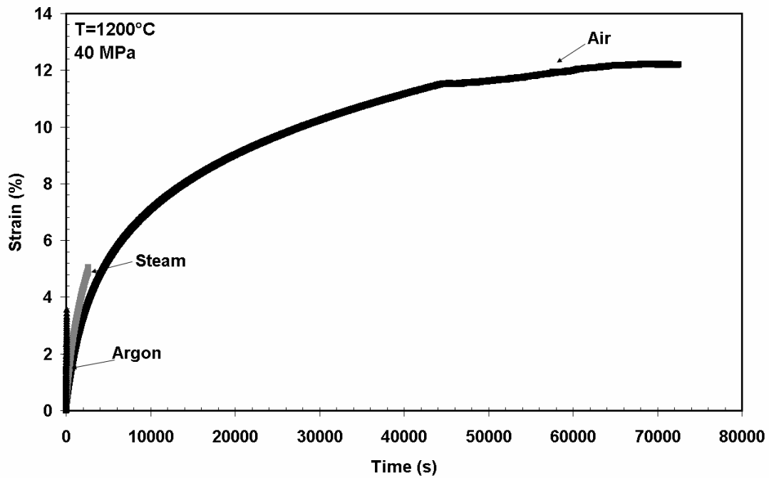
Figure 40. Creep strain vs. time obtained for creep stress of 40 MPa in air, steam, and argon environments at 1200°C.
