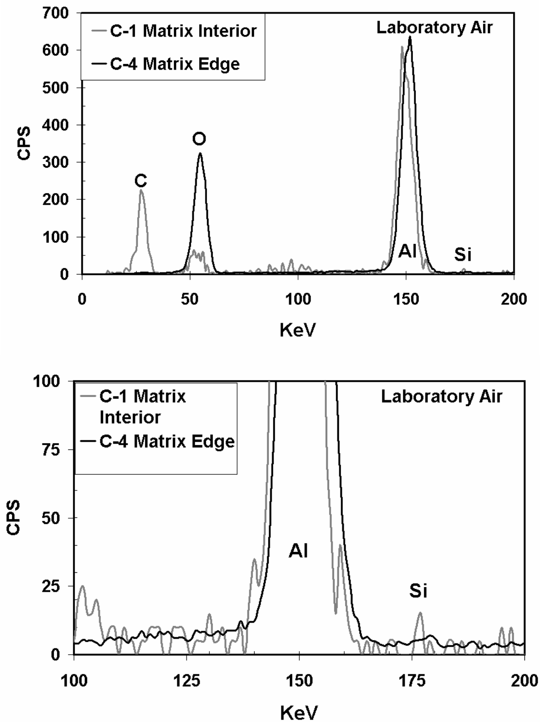
Figure 72. EDS spectra of the matrix interior compared to the spectra of the matrix edge in the specimens tested in laboratory air.
