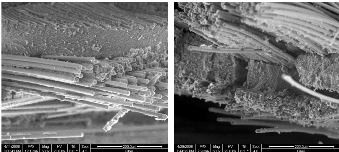
Figure 60. SEM micrographs depicting matrix failure between bundles.
