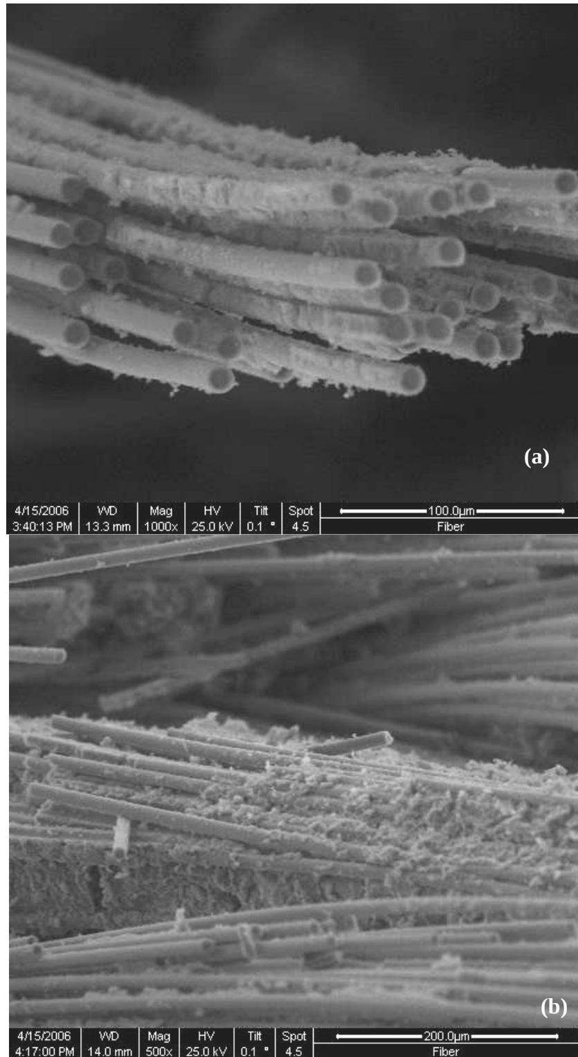
Figure 91. Micrograph of Nextel™ 720/alumina CMC specimen C-11 tested in creep at 40 MPa at 1200°C in 100% steam environment: (a) fiber bundle with individual fiber pullout, (b) breakdown of matrix separating fibers.
