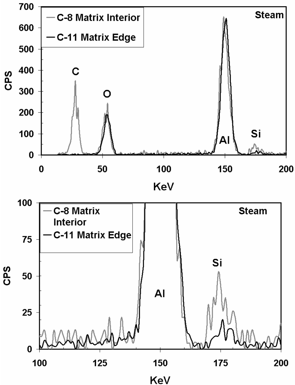
Figure 73. EDS spectra of the matrix interior compared to the spectra of the matrix edge in the specimens tested in 100% Steam.
