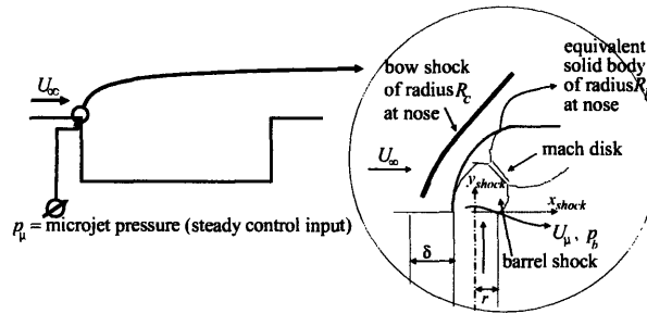
Figure 2-8: Close-up of flow structure near the exit of microjet nozzle in the presence of external cross-flow. Adapted from Papamoschou and Hubbard [16].
