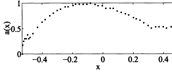
Figure 4-11: Radius profile of the store. Here x = \frac{\hat{x}}{\hat{t}_o} and a = \frac{\hat{a}}{\hat{t}_o} . Also x = 0 corresponds to the store c. g.
