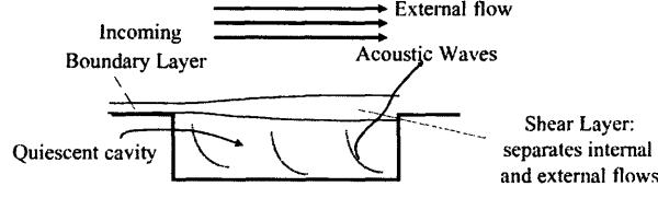
Figure 2-2: Illustration of the assumptions behind the reduced-order cavity acoustics model.
