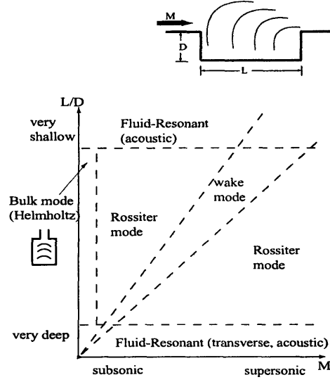
Figure 1-4: Different flow regimes seen by a cavity under external cross-stream.
