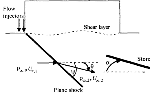
Figure 4-1: Shock geometry outside the cavity due to application of microjet-based flow injectors at the leading edge and upstream end.
