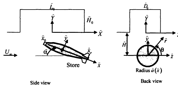
Figure N-1: Reference frames (both fixed to the store and inertial) for computing \hat{F} and \hat{M} on store.
