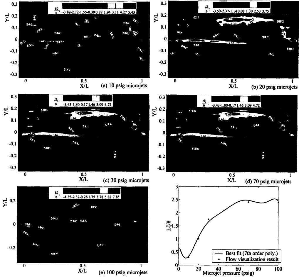
Figure D-1: Flow visualization results for the FSU cavity. Shown here are the mean transverse velocity gradient for different microjet pressures. Notation follows from Eqn. (D.7). The indicated box is the region of averaging for estimating the mean transverse microjet velocity gradient. External flow conditions: M = 2.0 and Re = 3 million (based on cavity length). Cavity dimension: L/D = 5.1 .
