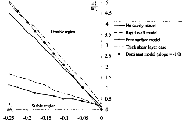
Figure 4-6: Stability region predicted by the five outside-cavity models in the no-control case. The initial conditions for the models are: Y_1 = \frac{\hat{V}_1}{\delta U_\infty} = -1.63 and \alpha_1 = \frac{\hat{\omega}_1}{\delta} = 0.01 with V_1 = \frac{\hat{V}_1}{\delta U_\infty} and \omega_1 = \frac{\hat{\omega}_1 l_c}{\delta U_\infty} shown in the above plot. The uncertainty in the stability boundaries are as follows: \Delta V_1 = \pm 0.005 , \Delta \omega_1 = \pm 0.125 . The cross-flow Mach number is 2.46, Reynolds number based on store length is 4.9 million, cavity aspect ratio is 5 and store length is half of cavity length.
