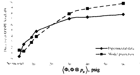
Figure 3-2: Model prediction versus experimentally observed OASPL reduction corresponding to the pressure transducer location at the middle of the trailing edge. External flow conditions: M = 2.0 and Re = 3 million (based on cavity length). Cavity dimension: L/D = 5.1 . The uncertainty in the pressure sensor reading was \pm 1.5dB and in frequency was \pm 40Hz . Also the initial conditions for determining d_\mu were: \frac{p'}{p} = 1.98 and \frac{\partial p'}{\partial t} = 0 (arbitrary).
