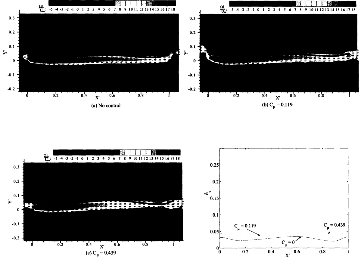
Figure G-1: Flow visualization results for the FSU cavity. Shown here is the shear layer shape for different microjet momentum ratios. The shear layer shape is indicated by a bold line in figures (a), (b) and (c). This line indicates the outer thickness of the shear layer (the side far from the cavity) that have non-negligible vorticity \Omega . Here L is the cavity length and U_\infty is the external undisturbed flow speed. The notations X' and Y' are explained in Eqn. (2.10). External flow conditions: M = 2.0 and Re = 3 million (based on cavity length). Cavity dimension: L/D = 5.1 .
