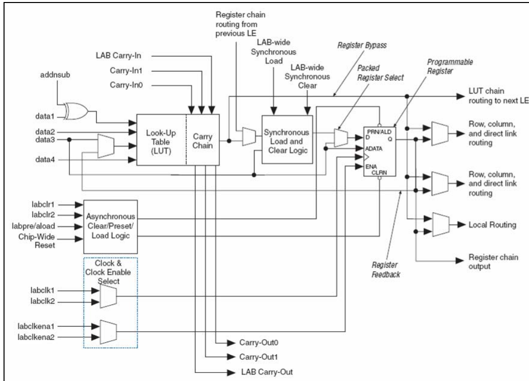
Figure 3. Altera Stratix Logic Element. This is one tenth of a Logic Array Block (Altera's nomenclature for a CLB). [Alt05]
