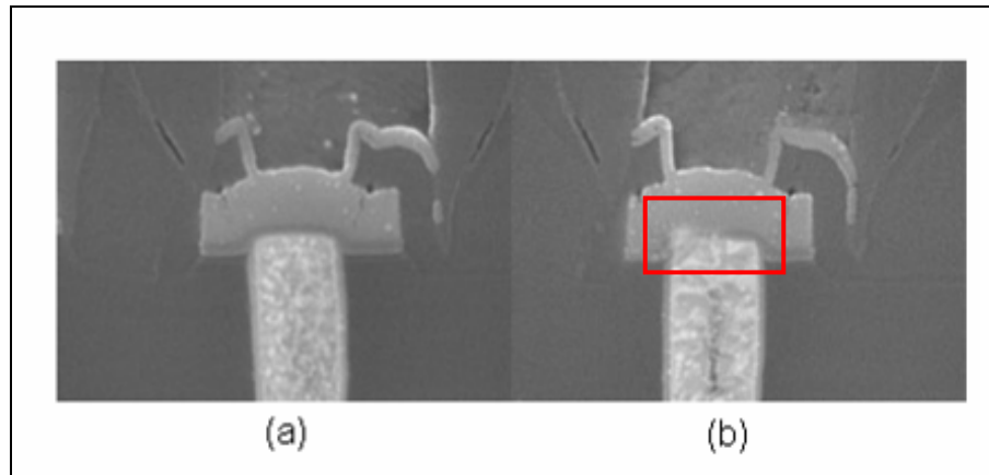
Figure 5. Cross sections of unprogrammed and programmed antifuses. [Act06]
