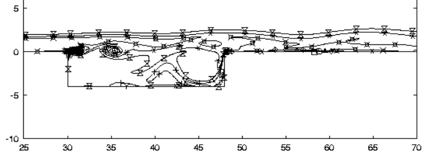
Figure 14: Contours of vorticity for a suboptimal forced flow. The freestream Mach number is M=0.85 . The mean blowing level is M=0.4 and harmonic forcing amplitude is M=0.2 and the frequency of forcing is 90% of the second Rossiter frequency (361 Hz). The contour levels are in increments of vorticity jumps of 2000/sec.
