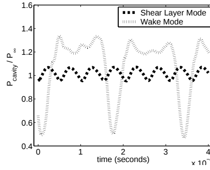
Figure 4: Traces of the time history of pressure on the downstream corner of the wall over several periods of natural oscillations.
