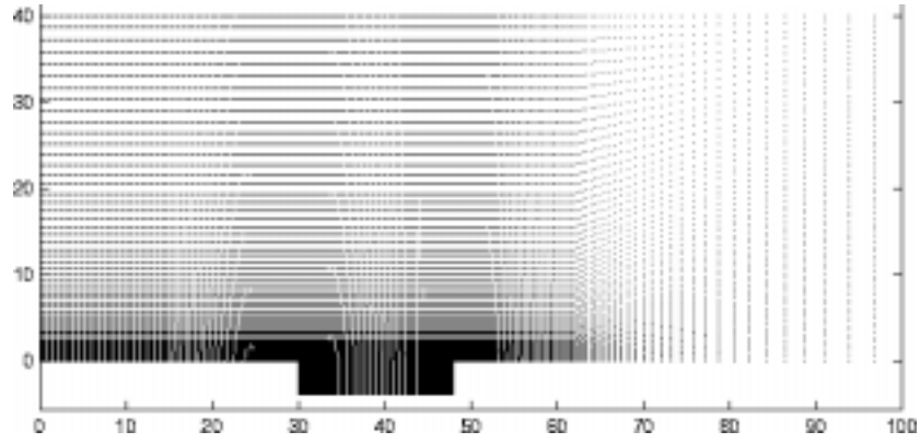
Figure 2: Two dimensional cavity grid generated by zone3g on an SGI.
