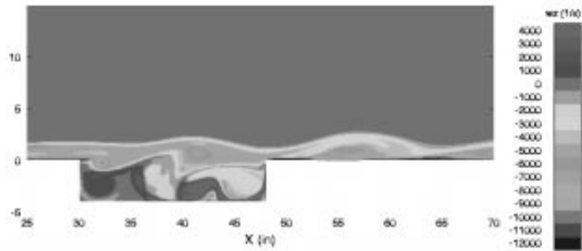
Figure 6: Vorticity contours in a snapshot of the fifth order spatial simulation of the shear layer mode behavior.
