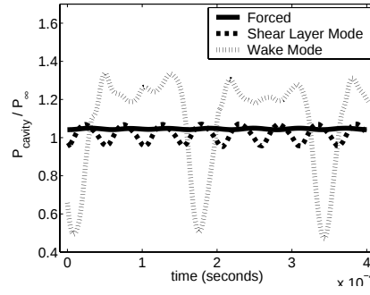
Figure 15: Traces of the times history of the pressure on the downstream corner of the wall.
