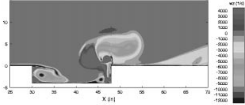
Figure 7: Vorticity contours in a snapshot of the fifth order spatial simulation of the wake mode behavior.
