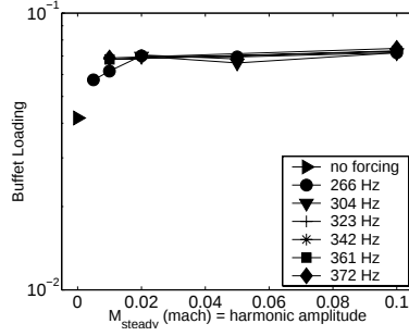
Figure 12: Buffet loading metric for several frequencies with harmonic forcing levels equal to the mean blowing Mach number.
