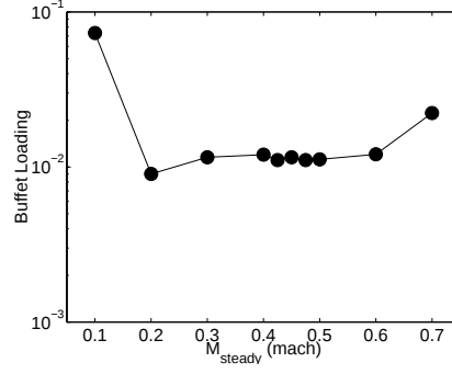
Figure 9: Buffet loading metric as a function of the mean blowing level for a harmonic forcing level of M=0.25 at a frequency of 90% of the second Rossiter frequency (361 Hz).
