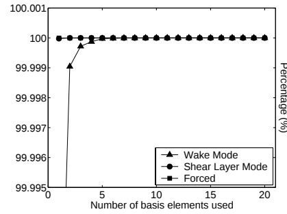
Figure 18: Measure of POD convergence based on relative 'energy' of pressure representation. The wake mode, shear layer mode, and forced case are the same as the cases in Figure 15.
