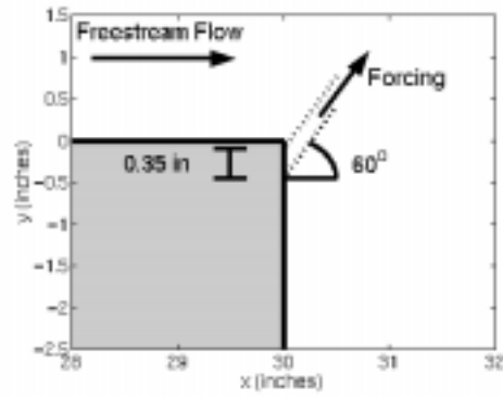
Figure 3: The location of the mean blowing and harmonic blowing slot indicated at the upstream cavity edge.
