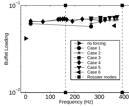
Figure 11: Buffet loading level at many frequencies with the harmonic forcing level equal to the mean blowing for Case 1, M=0.005 ; Case 2, M=0.01 ; Case 3, M=0.02 ; Case 4, M=0.05 ; Case 5, M=0.1 ; and Case 6, M=0.45 .
