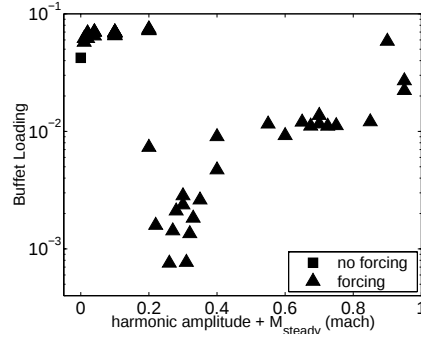
Figure 8: A simple presentation of the cases examined with buffet loading expressed as a function of the sum of mean and harmonic forcing Mach number.
