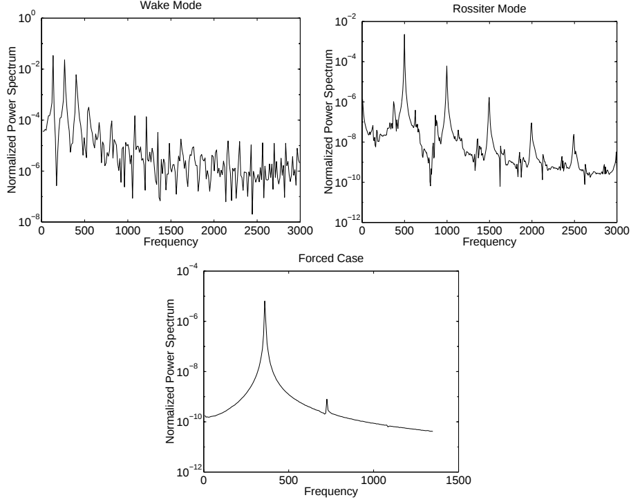
Figure 16: Spectra from the Wake Mode, Rossiter Mode, and Forced ( M_{steady} = 0.25 Mach, M_{harmonic} = 0.01 Mach, 361 Hz) cases.
