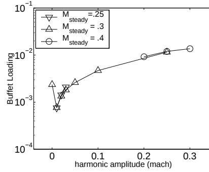
Figure 10: Behavior of the buffet loading metric at several harmonic forcing amplitudes for mean blowing levels of M=0.3 and M=0.4 and frequency of Figure 9.
