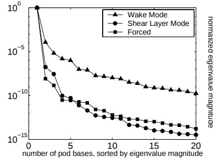
Figure 17: Distribution of normalized amplitudes of POD elements. The wake mode, shear layer mode, and forced case are the same as the cases in Figure 15.
