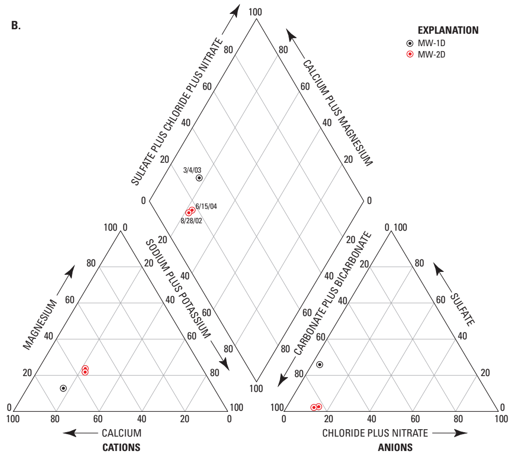
Figure 37. The water chemistry of samples from (A) regolith and transition-zone wells and the lake site, and (B) open-borehole bedrock wells at the Langtree Peninsula research station, North Carolina.
