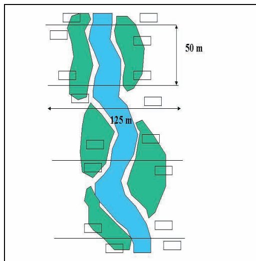
Figure 3. An example of a randomized sampling approach, where sampling quadrats are located randomly along transects. Transects should be spaced approximately 50 m apart and should be long enough to cover the width of the riparian zone (Stromberg 2000a)
