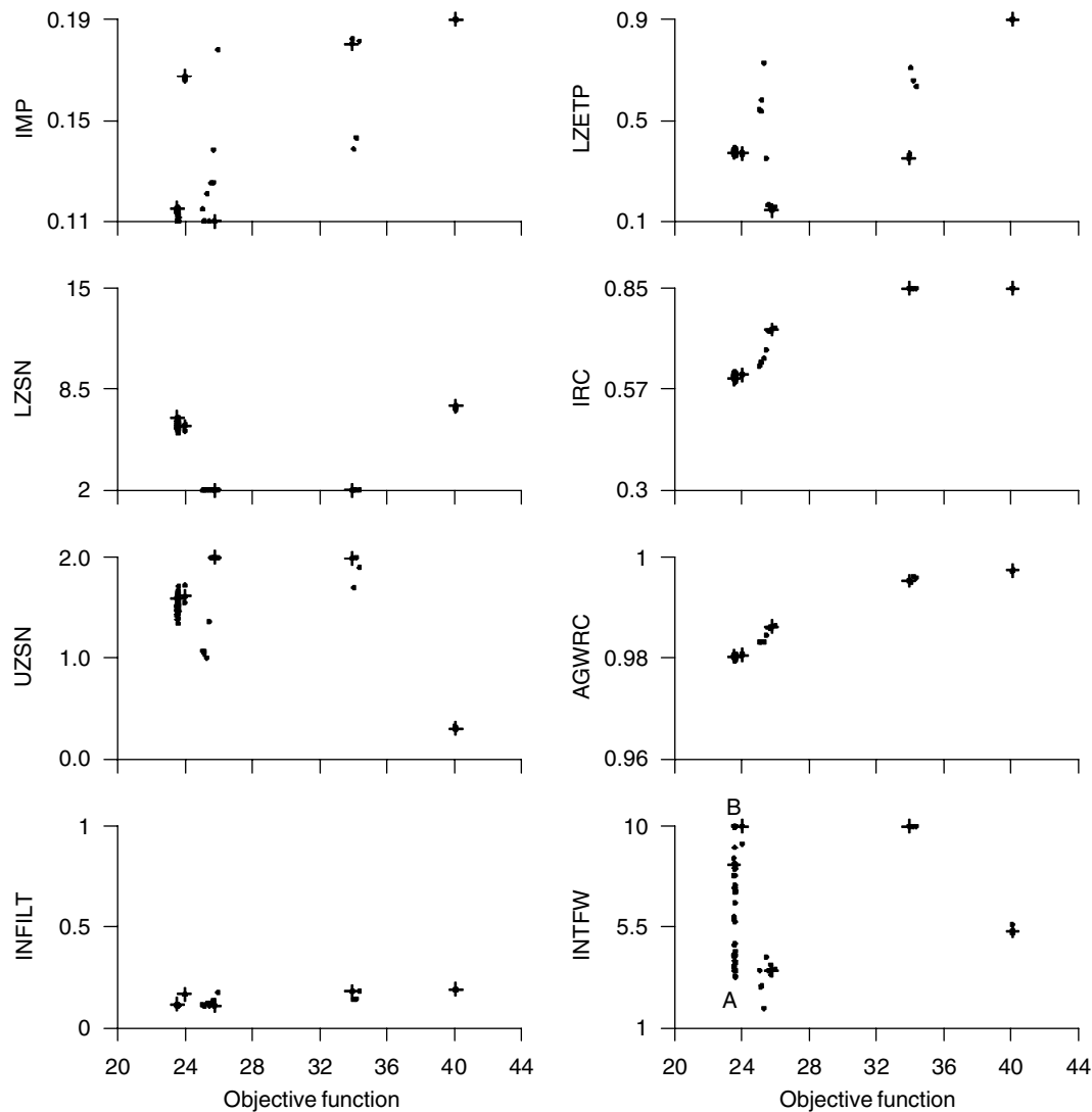
Figure 3 End-points in parameter space of 100 PEST runs undertaken under the control of PD_MS2. Parameters comprising an optimized set are linked vertically between graphs by objective function. PEST's TPI functionality was operative. Crosses mark the breakpoints of the objective function traverse depicted in Fig. 5.
