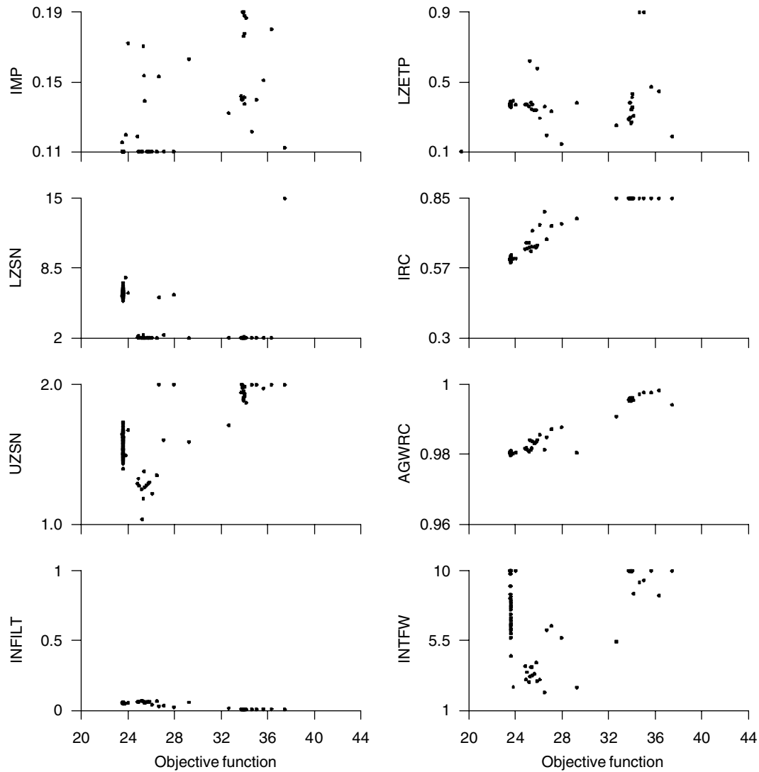
Figure 2 End-points in parameter space of 100 PEST runs undertaken under the control of PD_MS2. Parameters comprising an optimized set are linked vertically between graphs by objective function. PEST's TPI functionality was not operative.
