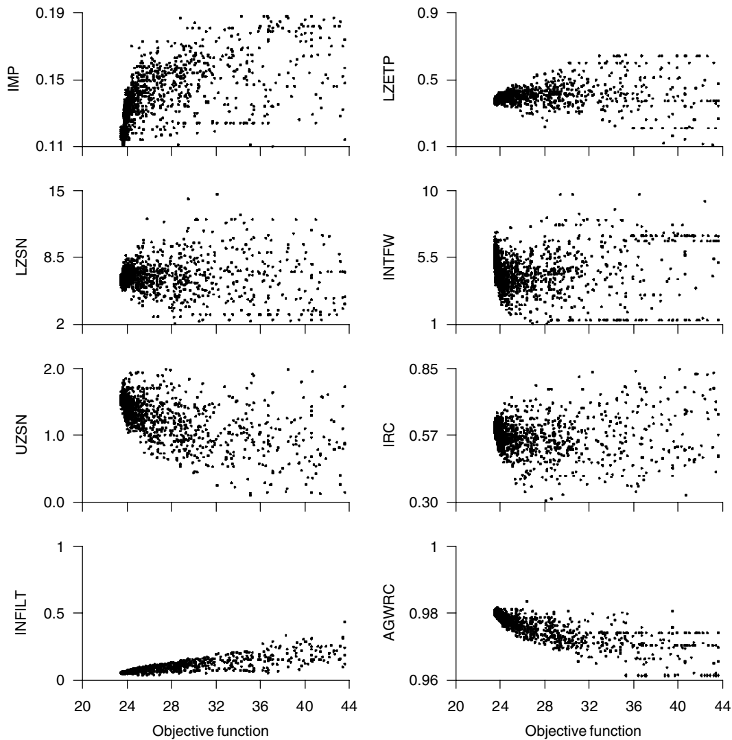
Figure 8 Best parameters and objective functions obtained by SCE-UA at the end of each shuffling loop of the 8-parameter calibration problem. (Note that only objective functions below 44.0 are represented in this figure; the objective function at the commencement of the parameter estimation process was over 200.)
