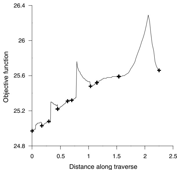
Figure 6 Objective function along traverse between parameter sets marked with crosses in the first frame of Fig. 4. These same parameter sets are also shown as crosses in the transect.
