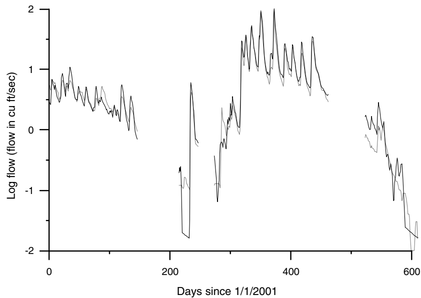
Figure 1 Observed (dark) and modeled (light) daily flows corresponding to global objective function minimum.
