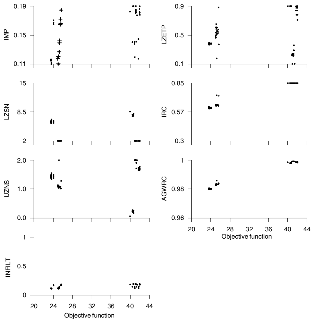
Figure 4 End-points in parameter space of 100 PEST runs undertaken under the control of PD_MS2 with INTFW fixed at 3.4. Parameters comprising an optimized set are linked vertically between graphs by objective function. PEST's TPI functionality was operative. Crosses (only shown for first frame of this figure) mark the breakpoints of the objective function traverse depicted in Fig. 6.
