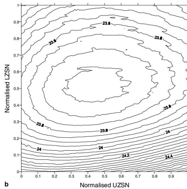
Figure 7 (a) Objective function surface computing by varying UZSN and LZSN incrementally about their optimized values and sampling at small, regular intervals. (b) Objective function contours corresponding to (a).
