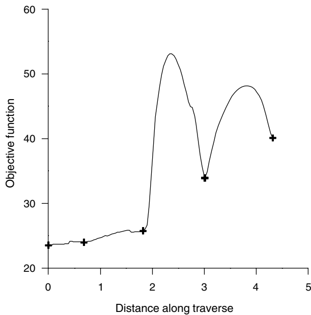
Figure 5 Objective function along traverse between parameter sets marked with crosses in Fig. 3. These same parameter sets are also shown as crosses in the transect.
