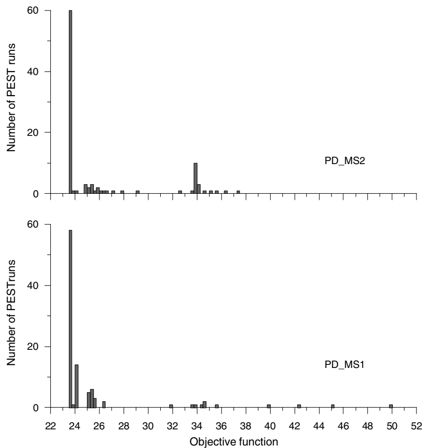
Figure 9 Objective function occurrences for 100 PEST runs based on random starting locations (lower figure), and starting locations selected during a single, long, PD_MS2 run (upper figure).
