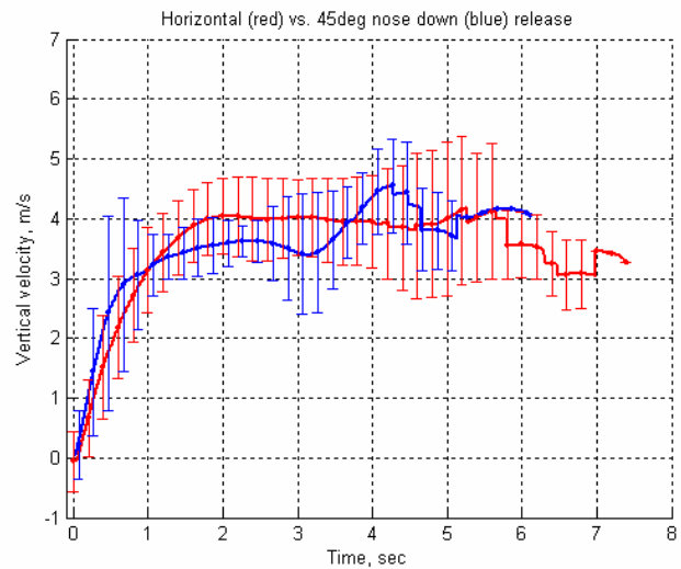
Fig. 7. Average velocity in drops with release pitch at horizontal and 45 deg nose down
