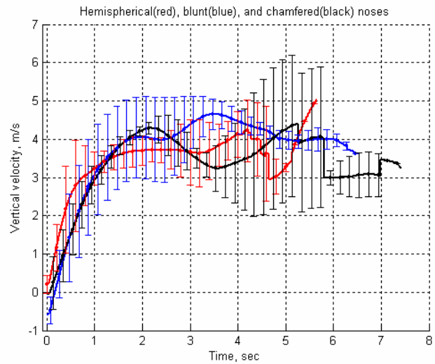
Fig. 6. Average vertical velocity in drops with three different nose types: hemispherical, blunt, and chamfered
