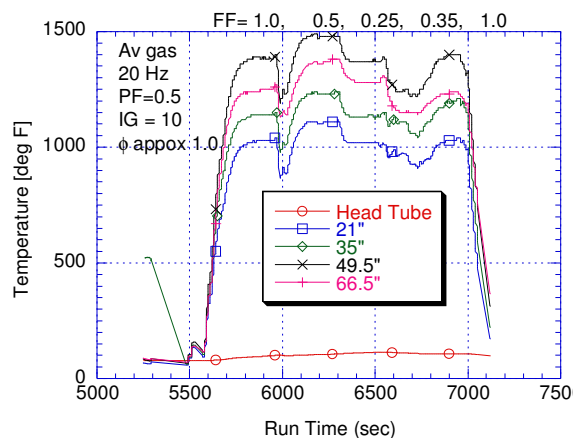
Figure 6. Detonation tube temperatures verses run time for several fill fractions, 72" (1.83m) detonation tube
