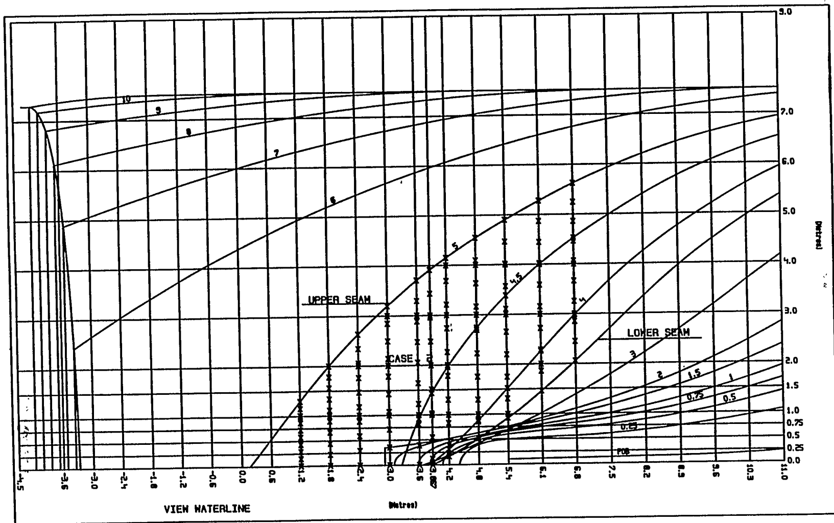
FIGURE 6.3.5 - SELECTED TEST CASE 2 - WATERLINES
