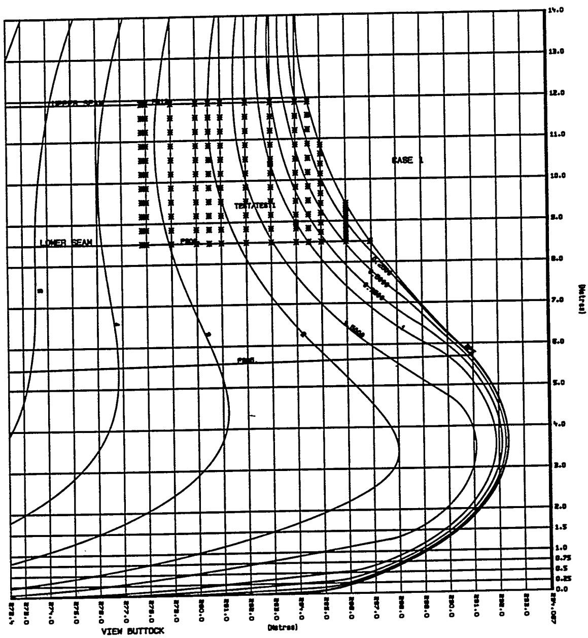
FIGURE 6.3.3 - SELECTED TEST CASE 1 - BUTTOCKS
