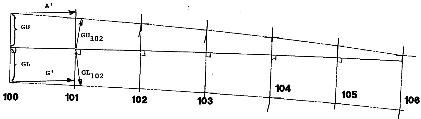
FIGURE 1.4.4.2 - CENTER SQUARING OFF METHOD SHELL PLATE EXPANSION
