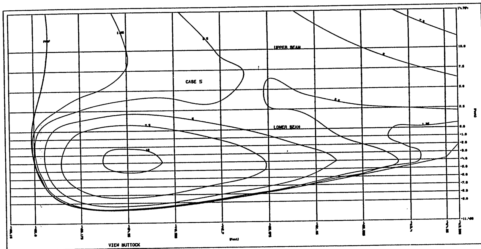
FIGURE 6.3.12 - SELECTED TEST CASE 5 - BUTTOCKS
