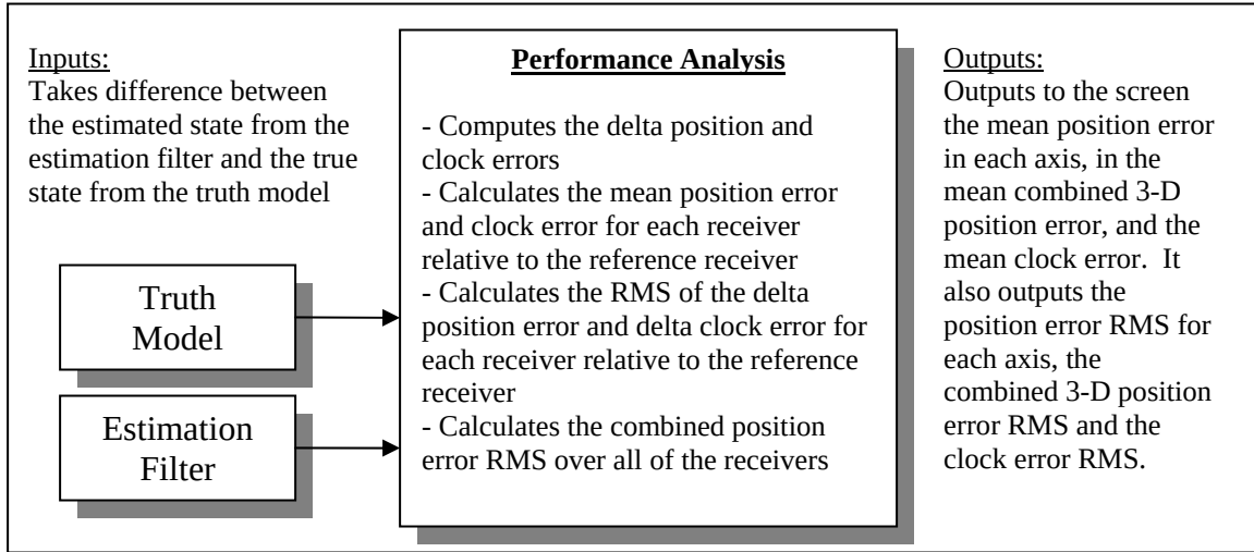
Figure 3.7.1 Block Diagram of the Performance Analysis Function
