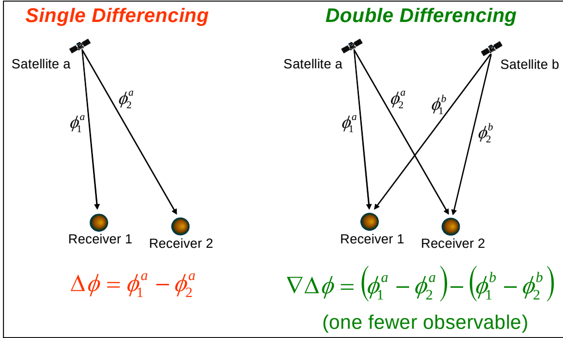
Figure 2.2.4 Differential GPS [37]
