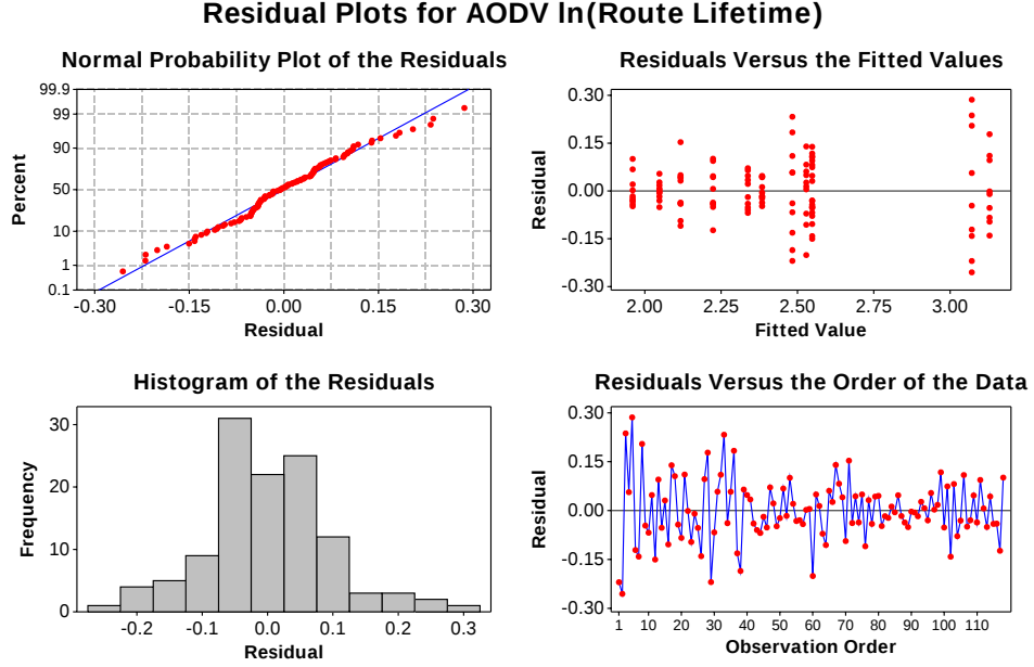
Figure C.2: Residual Plots for AODV \ln(\text{Route Lifetime})
