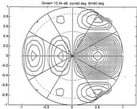
Figure 5 16-element array composite beam pattern
