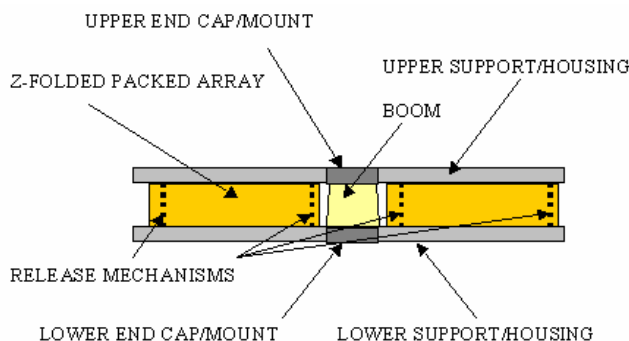
Figure 6: Stowed Configuration
