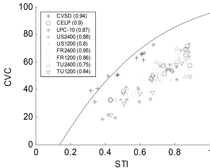
Figure 3. Scatter plot of speech-based STI using noise suppression correction with corresponding CVC scores. Solid line and numerical values as in Figure 2.
