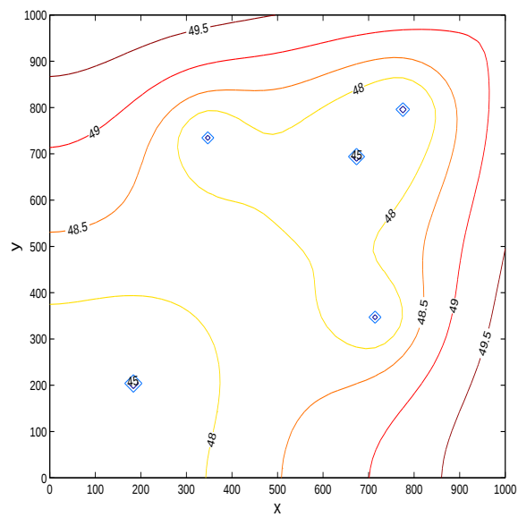
Figure 4. Initial Iterate
