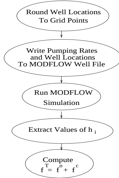
Figure 2. Objective Function Evaluation
