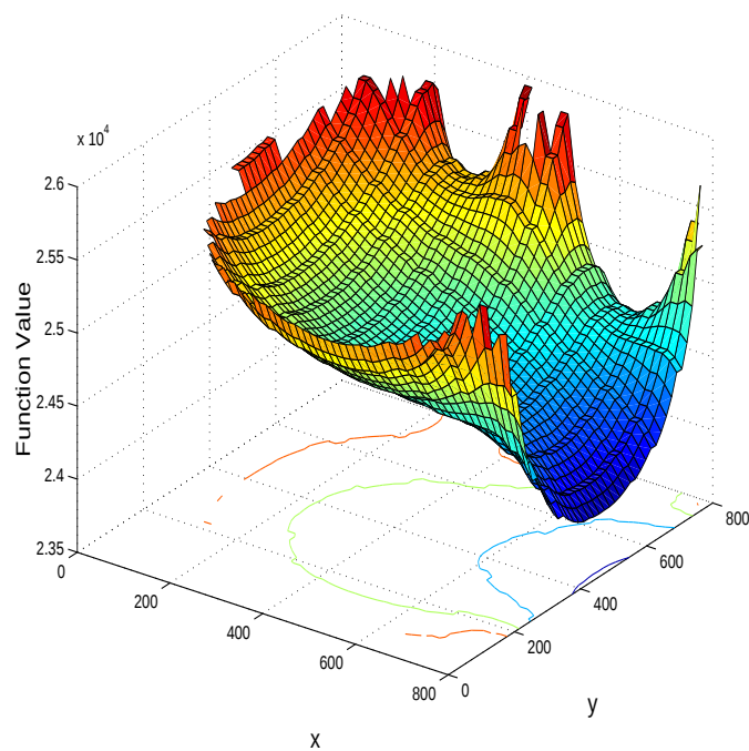
Figure 11. Landscape near solution: unconfined aquifer
