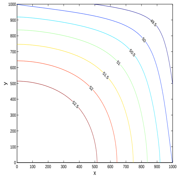
Figure 3. Steady state head, confined aquifer
