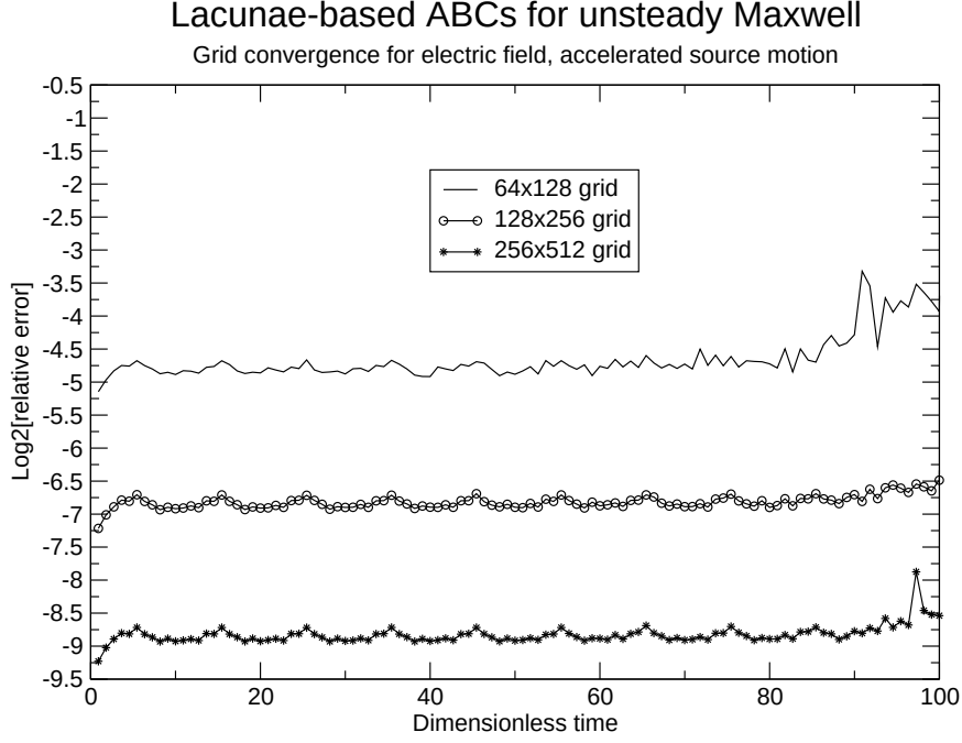
Fig. 3. Grid convergence study with lacunae-based ABCs, \varepsilon = 8\Delta r .
