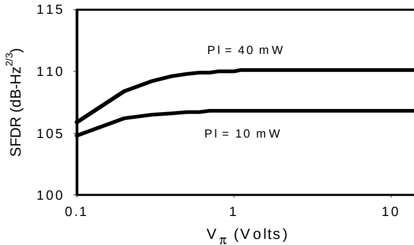
Figure 6. SFDR of a MZM as a function of V_\pi .
