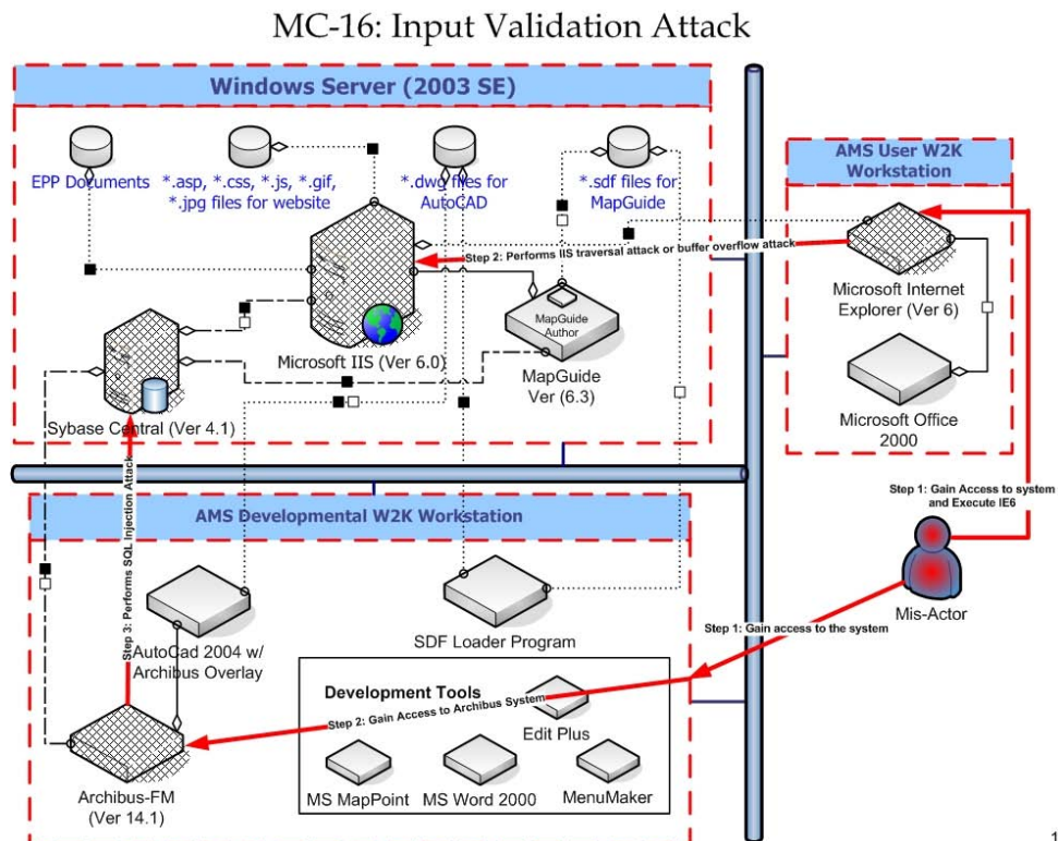
Figure 13: Sample Final Version of a Misuse Case Diagram
