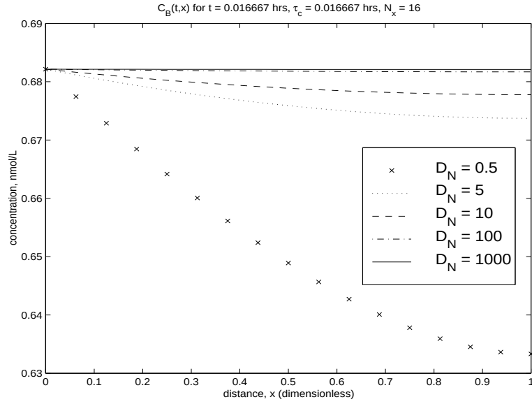
Figure 11: Predicted concentrations of TCDD in the liver blood compartment as a function of distance, x , and the axial dispersion number, \mathcal{D}_N , at time t = 1 minute.
