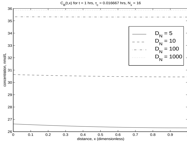
Figure 12: Predicted concentrations of TCDD in the liver blood compartment as a function of distance, x , and the axial dispersion number, \mathcal{D}_N , at time t = 1 hour.
