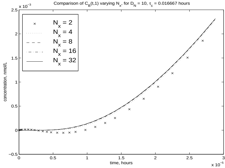
Figure 3: Numerical solution for C_B(t, 1) varying the number of basis elements, N_x , with \mathcal{D}_N = 10 . The solutions with N_x = 8, 16 , and N_x = 32 are identical on this scale, indicating convergence of the Galerkin approximations with 8 basis elements.
