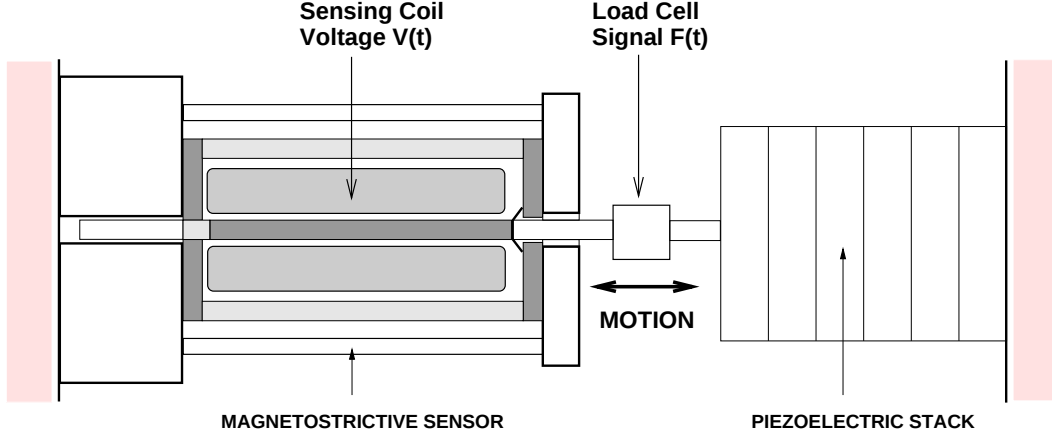
Figure 2: Schematic representation of the assembly used to drive the magnetostrictive sensor. Measured input was driving force F(t) , while measured output was sensing voltage V(t) .
