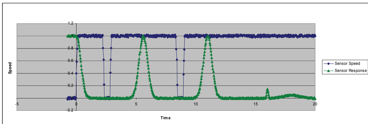
Figure 7. Idealized corrected sensor speed and sensor response versus time.
