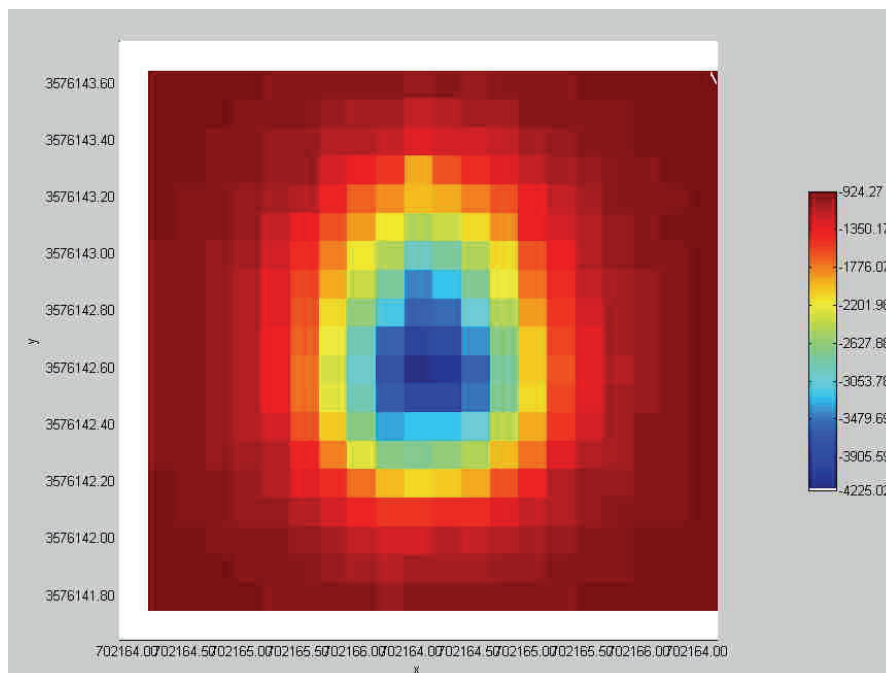
Figure 13. Data taken on the UXO/CM test stand using the GEM-3-E.
