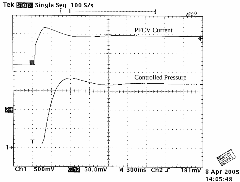
4.0. Flight Xenon Feed System Response/Steady State with Xenon at 1200 psia With Breadboard PI Controller
