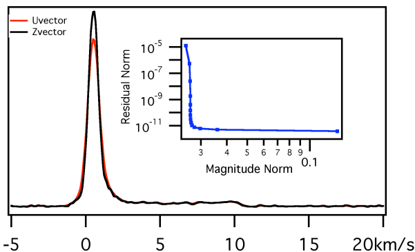
Fig. 6. Radial LIF profile (U vector) 28 mm downstream of exit plane, and resulting deconvolved VDF (Z vector). Also shown is the L-curve computed. Note the sharpening of the peak due to deconvolution is significant due to the relatively narrow distribution relative to the PSF.
