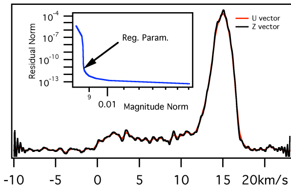
Fig. 5. Exit plane axial LIF profile (U vector), and resulting deconvolved VDF (Z vector). Also shown is the L-curve computed with the location of regularization parameter used. Note the small difference between VDF and LIF profile
