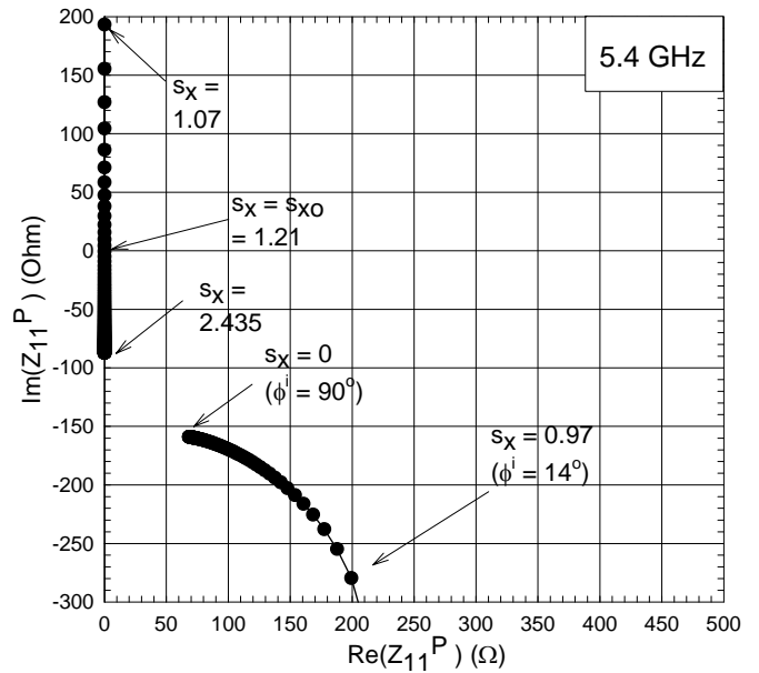
Figure 2- The self impedance of an infinite planar array of dipoles as the phase between successive columns is changed varied between 0 and 180 Degrees.
