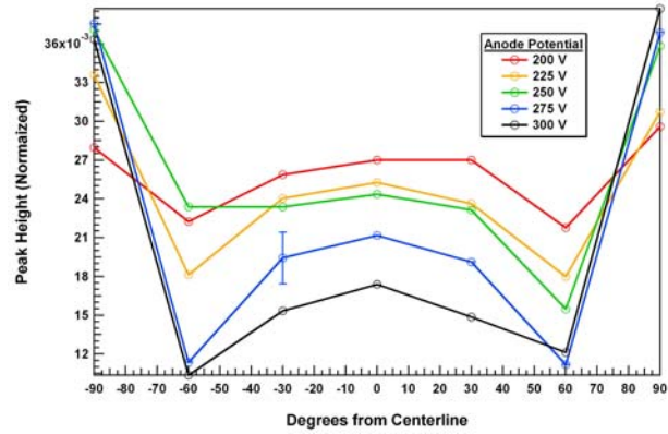
Figure 11. Ion Energy Peak Magnitude Relationship to Plume Angle. Note the rapidly increasing signal strength at the highly oblique angles, > \pm 60^\circ from thruster centerline.
