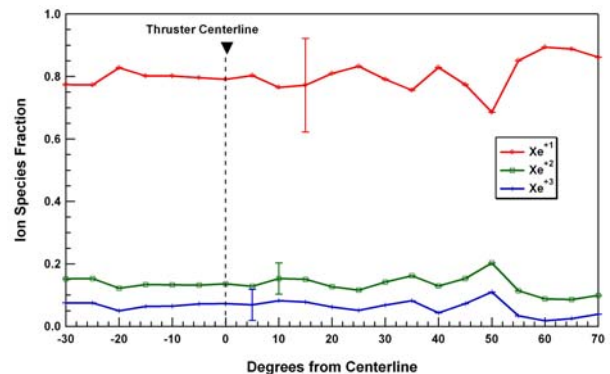
Figure 13. Ion Species Trends. Note relative consistency of ion species fraction measurements throughout the plume.
