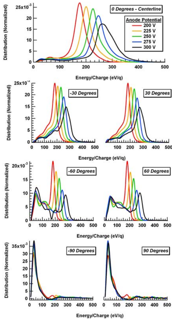
Figure 10. Energy Distribution Measurements. The increase ion scattering can be seen as the secondary peak become more prominent further away from centerline. Note symmetry agreement between measurements.
