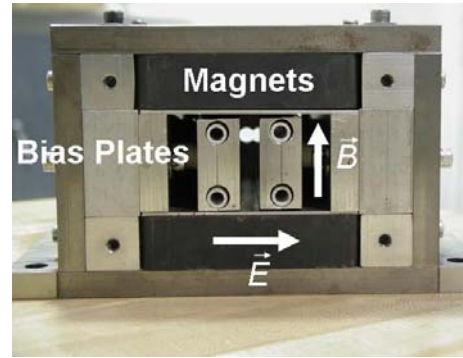
Figure 4. ExB Probe with front plate removed. Note orientation of magnetic and electric field within the test section with the front plate removed.
