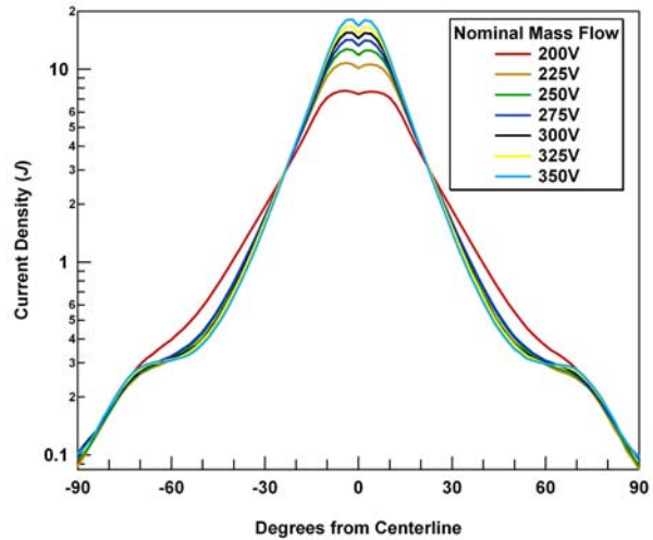
Figure 7. Faraday Cup Measurements. Note presence plume wings at greater than 60^\circ .
