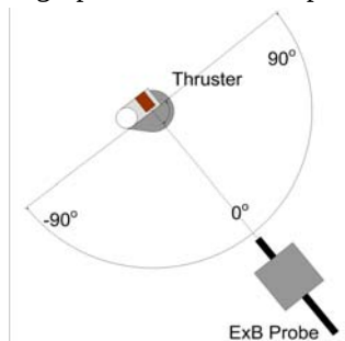
Figure 5. Chamber 6 Setup for ExB Probe measurements. Due to chamber and probe dimensions only angles -30^\circ through 70^\circ were investigated.
