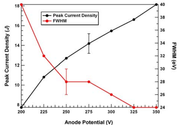
Figure 9. Peak Current Density and FWHM. Note inverse relationship on plume broadening with increasing anode potential and current density at nominal mass flow rates.
