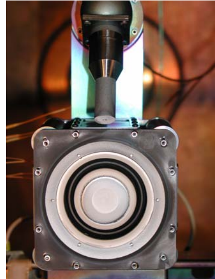
Figure 1. Busek BHT–HD–600 Hall thruster. Busek’s 600 W Hall thruster has been identified as a candidate for future microsatellites due to its high performance and modest power consumption.
