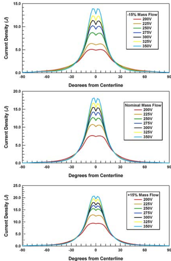
Figure 8. Current Density, J , - Mass Flow Relationships. Faraday Cup probe traces: -15%, nominal and +15% flow rates.
