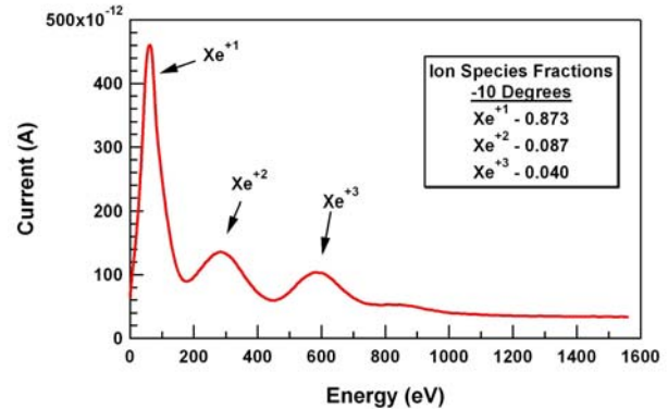
Figure 12. Typical E x B Trace. Note distinct peaks for three ion species indicating presence of Xe^{+1} , Xe^{+2} and Xe^{+3} . Note: calculated energy values are incorrect.
