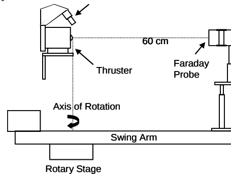
Figure 6. Chamber 6 Setup for Faraday and RPA Measurements. Thruster setup was centered on chamber axis achieving scanning capability of \pm 90^\circ .
