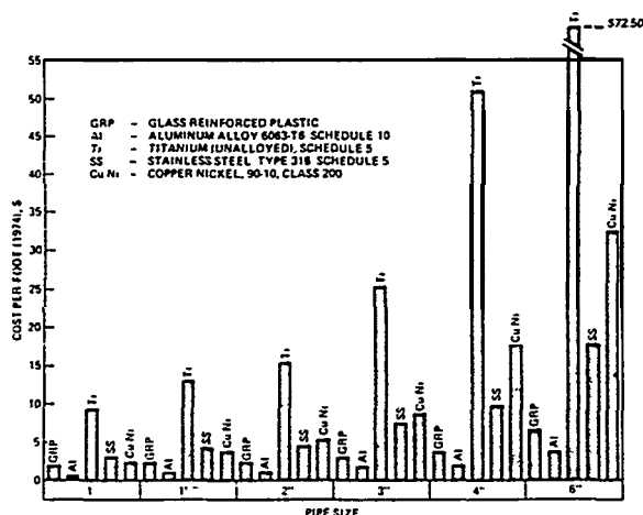
Figure 3. Coat Comparison of Various Piping Materials.
