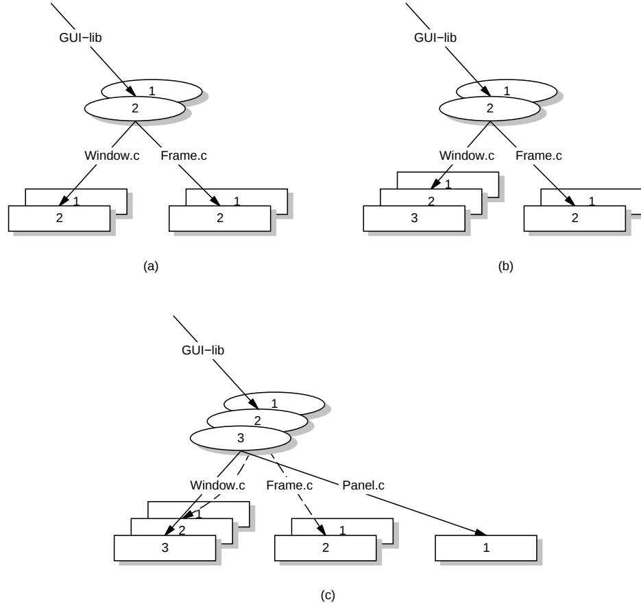
Figure 5: Progressive States of an Example Collection.
