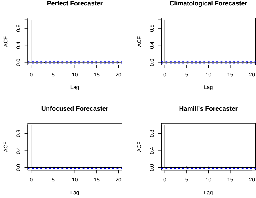
Figure 2: Sample autocorrelation functions for the probability integral transform.
