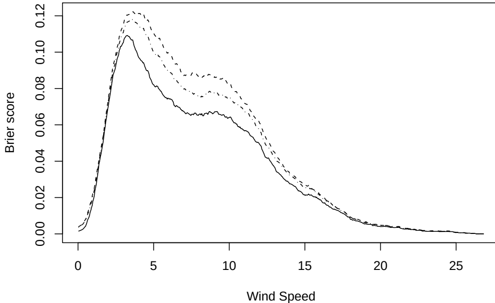
Figure 12: Brier score plot for persistence forecasts (dashed line), autoregressive forecasts (dot-dashed line) and RST forecasts (solid line) of hourly average wind speed at the Stateline wind energy center, in \text{m}\cdot\text{s}^{-1} . The graphs show the Brier score as a function of the threshold value. The area under the associated curve equals the CRPS value (14).
