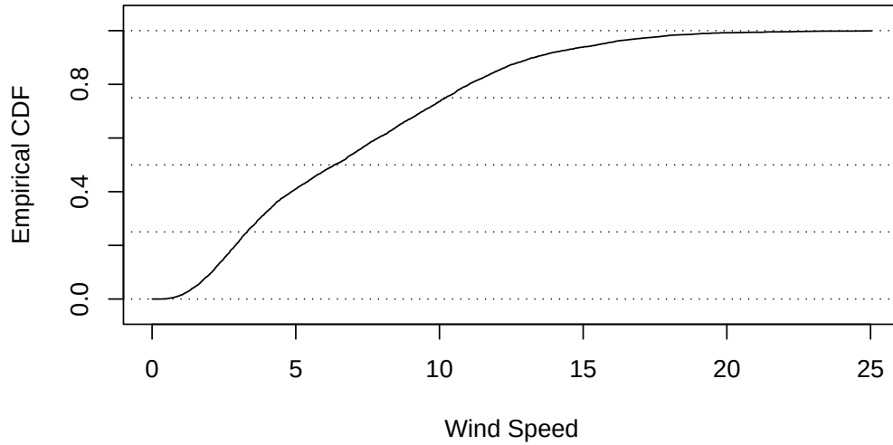
Figure 10: Empirical cumulative distribution function of hourly average wind speed at the Stateline wind energy center in May through November 2003, in \text{m} \cdot \text{s}^{-1} .
