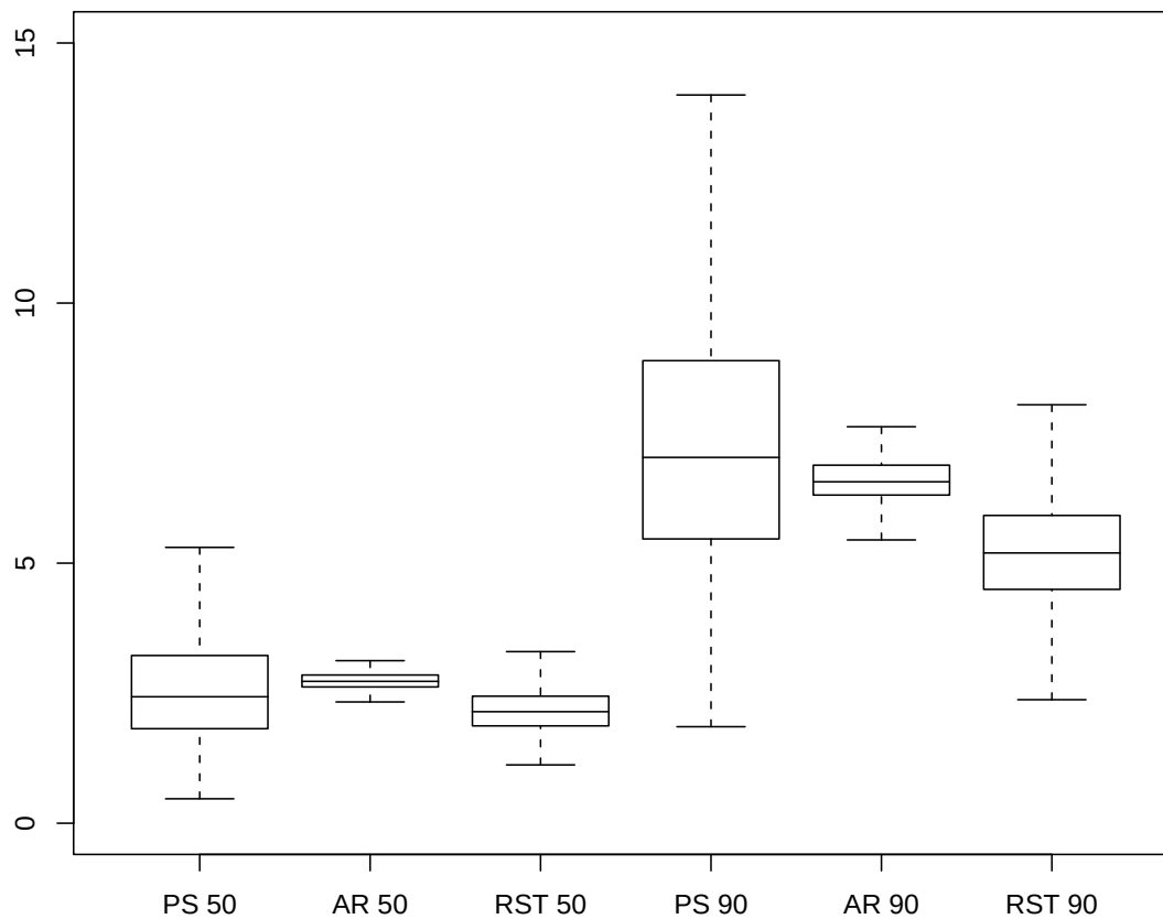
Figure 11: Sharpness diagram for persistence forecasts (PS), autoregressive forecasts (AR) and RST forecasts of hourly average wind speed at the Stateline wind energy center. The boxplots show the 5th, 25th, 50th, 75th and 95th percentile of the width of the central prediction interval, in \text{m} \cdot \text{s}^{-1} . The nominal coverage is 50% and 90%, respectively.
