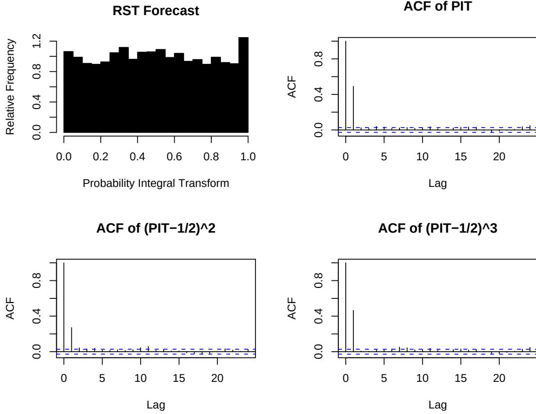
Figure 8: Same as Figure 6, but for RST forecasts.
