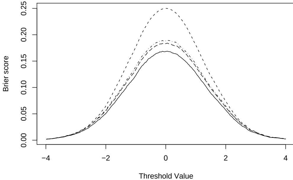
Figure 5: Brier score plot for the perfect forecaster (solid line), climatological forecaster (short dashes), unfocused forecaster (dot-dashed line), and Hamill’s forecaster (long dashes). The graphs show the Brier score as a function of the threshold value. The area under the associated curve equals the CRPS value (14).
