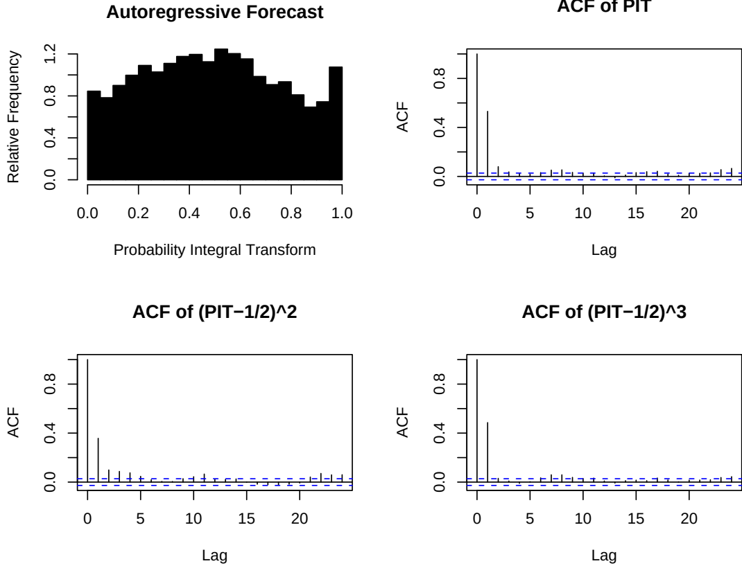
Figure 7: Same as Figure 6, but for autoregressive forecasts.
