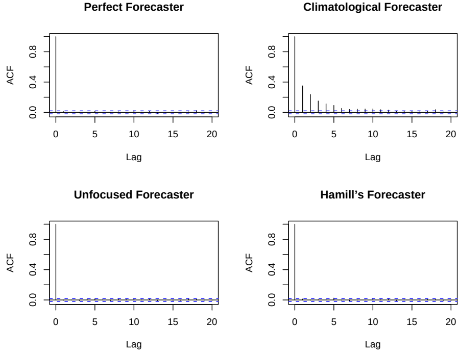
Figure 3: Same as Figure 2 except that the states, \mu_t , are now serially dependent, following a stationary Gaussian autoregression of order 1 with autoregressive parameter \frac{1}{2} .
