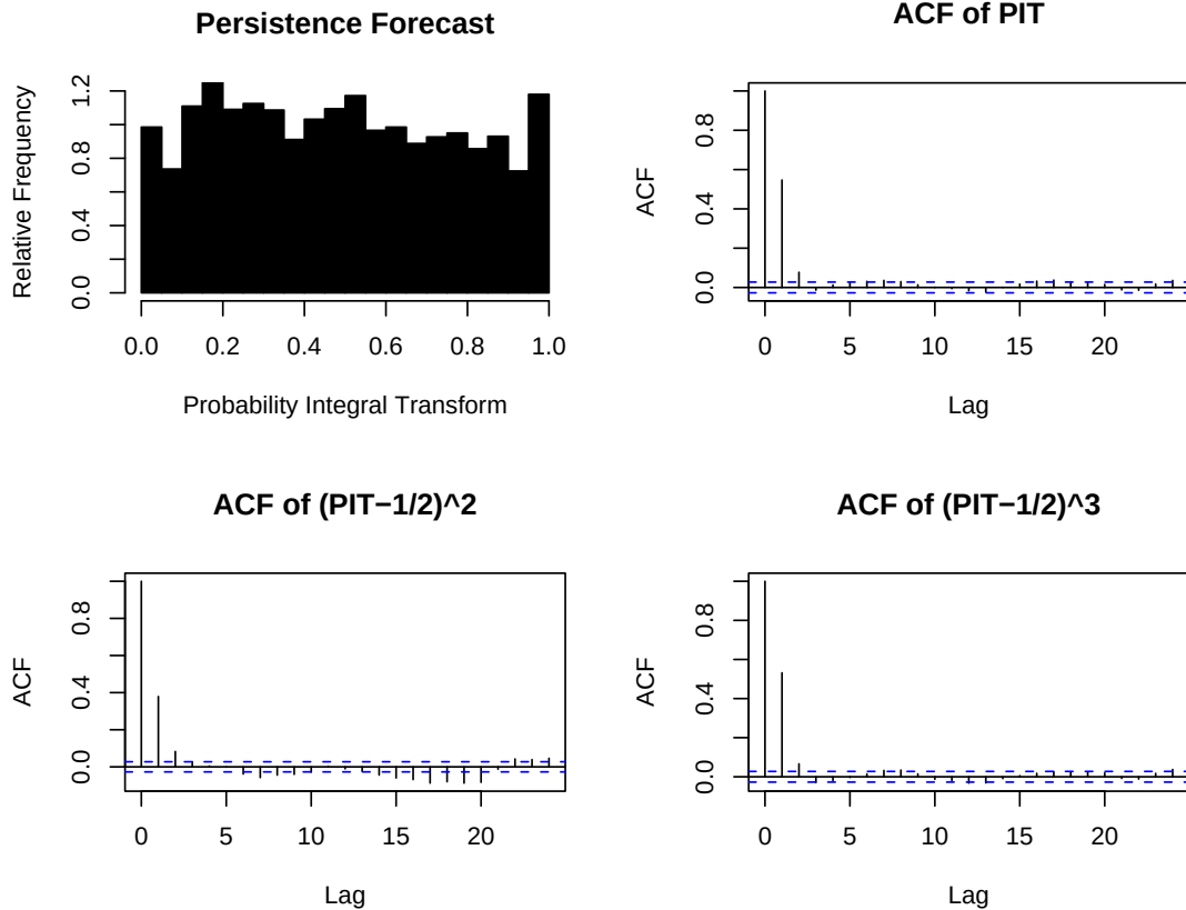
Figure 6: Probability integral transform (PIT) histogram and sample autocorrelation functions for the first three centered moments, for persistence forecasts of hourly average wind speed at the Stateline wind energy center.
