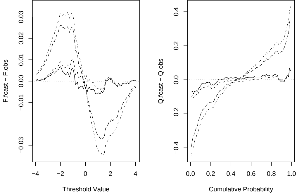
Figure 4: Marginal calibration plot for the perfect forecaster (solid line), climatological forecaster (short dashes), unfocused forecaster (dot-dashed line) and Hamill’s forecaster (long dashes). The presentation is in terms of cumulative distribution functions (left) and in terms of quantiles (right), respectively.
