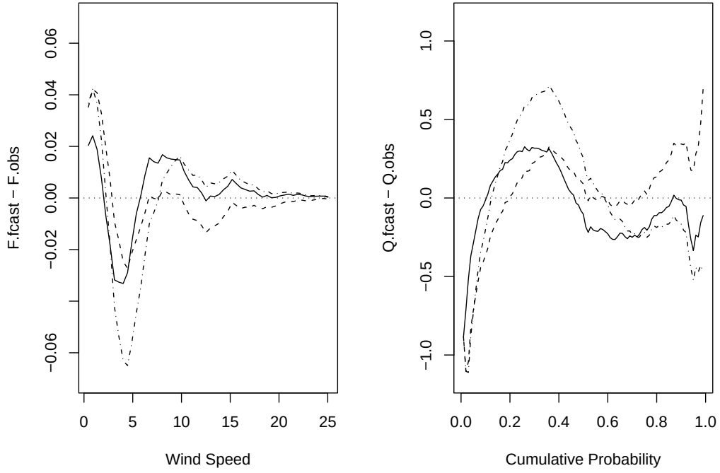
Figure 9: Marginal calibration plot for persistence forecasts (dashed line), autoregressive forecasts (dot-dashed line) and RST forecasts (solid line) of hourly average wind speed at the Stateline wind energy center in terms of cumulative distribution functions (left) and in terms of quantiles (right), respectively, in \text{m} \cdot \text{s}^{-1} .
