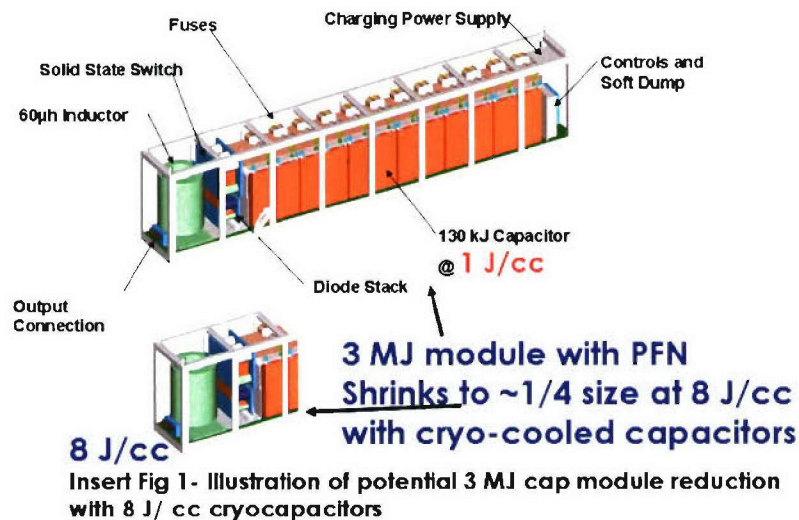
Fig. 2-1. Potential advantages of a 8 J/cc for a 3 MJPFN module
