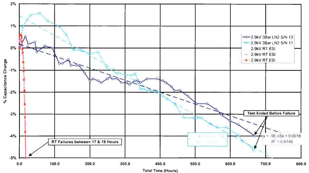
Fig. 7-14. DC life test results
