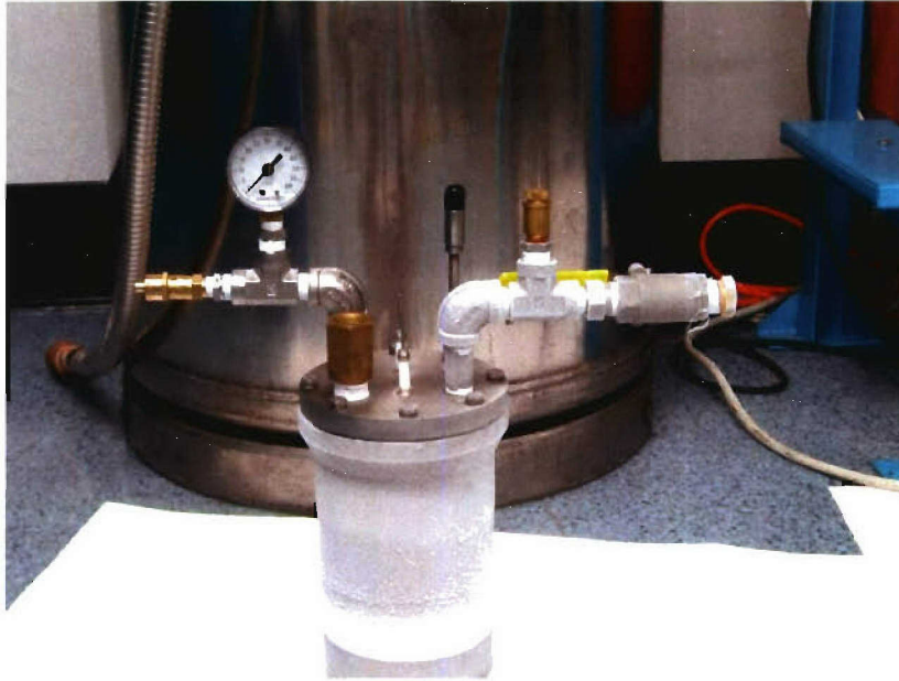
Fig. 5-4. Photograph of a reusable cryogenic test vessel being pressure-tested
