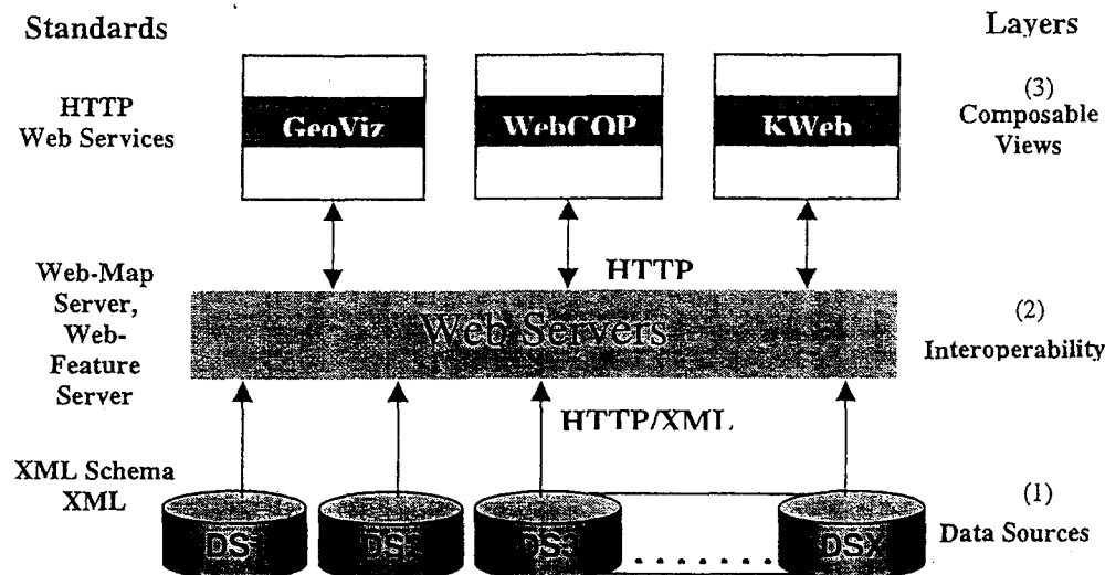
Fig. 2. Modular and flexible architecture of Phase I consisting of multiple data sources, views, standards and layers to support users of the Common Operating Picture (COP).
