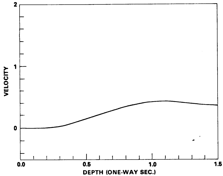
Figure 3: Velocity trend perturbation.
