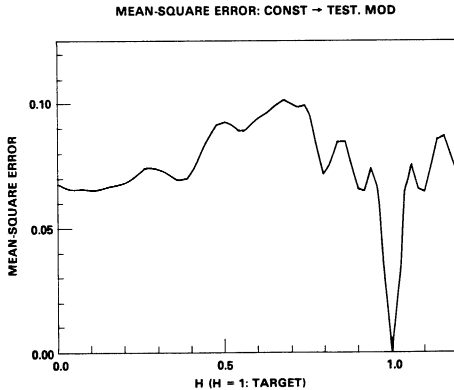
Figure 4: Scan of mean-square error over line segment connecting constant background velocity with that displayed in Fig. 1.
