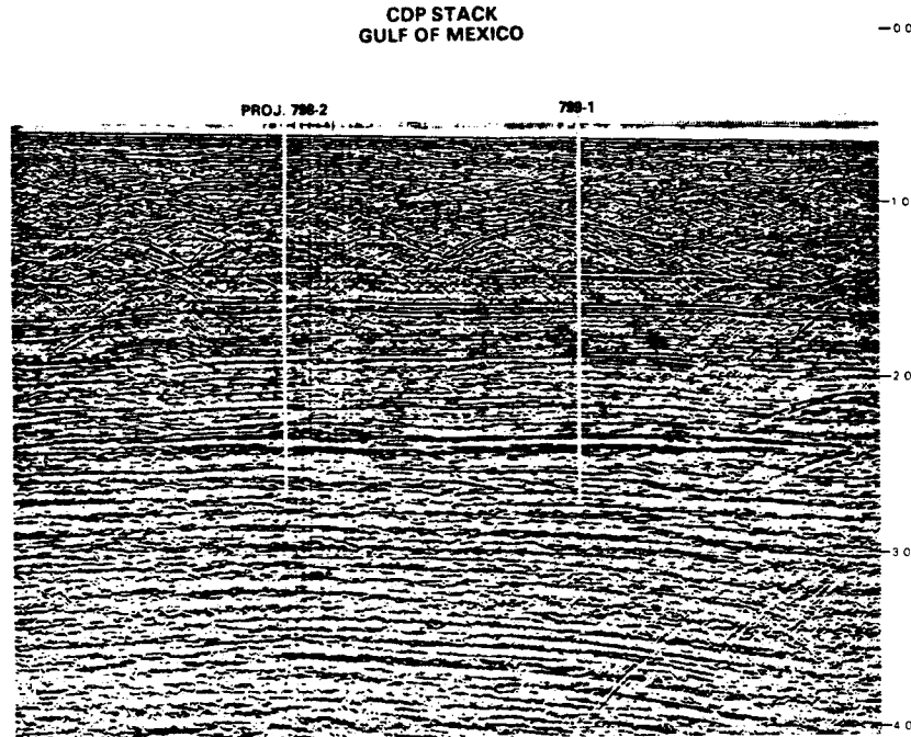
Figure 13: Gulf of Mexico data: CDP stack.
