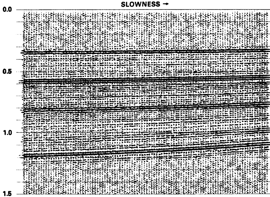
Figure 10: Data with 50% RMS pseudorandom passband noise.
