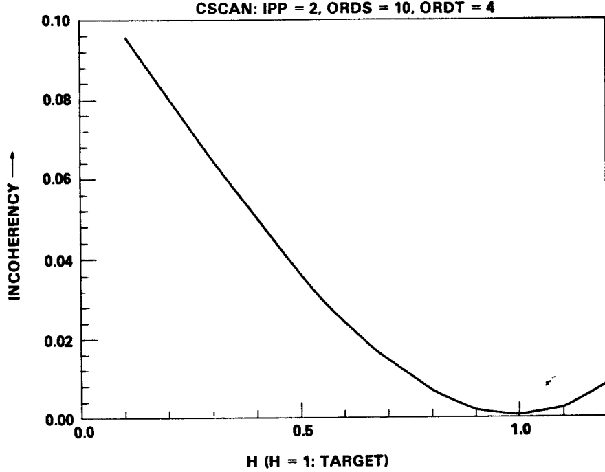
Figure 5: Scan of incoherency W over the same segment of velocity models as used to produce Fig. 4.
