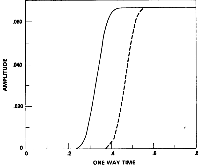
Figure 6b: Integrated cubic b-splines.
