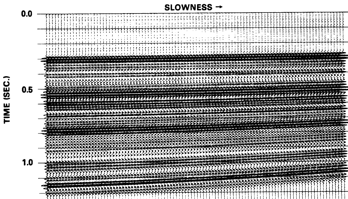
Figure 12: Final reflectivity estimate corresponding to Fig. 11.
