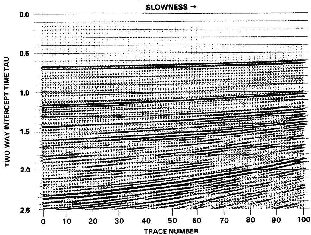
Figure 15: Gulf of Mexico data: windowed, deghosted, filtered, and resampled version of Figure 14. Input data for inversion.
