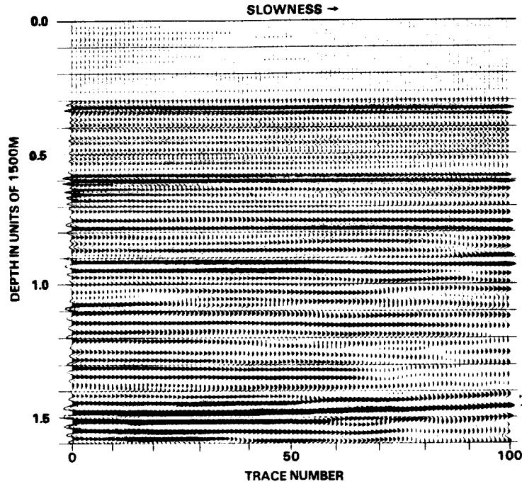
Figure 17: NMO corrected reflectivity corresponding to results of Fig. 16.
