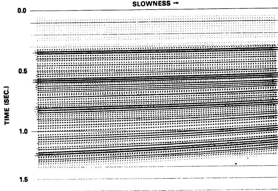
Figure 2: Convolutional plane-wave seismogram corresponding to the model of Fig. 1.
