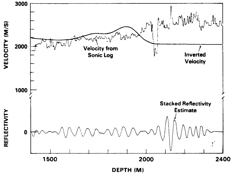
Figure 16: Results of inversion: top curves are velocity estimate (smooth curve) and interpreted sonic log (ragged curve). Bottom curve is stacked reflection series estimate. Products of 10 Gauss-Newton steps.
