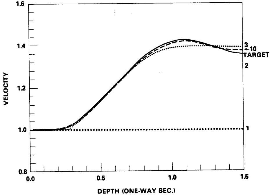
Figure 7a: Estimated velocity. 10 Gauss/Newton/trust region steps; constant initial velocity, zero initial reflectivity. Shown are the target (solid line) and iterates 1, 2, 3, and 10. Note that the general trend is achieved in three steps.
