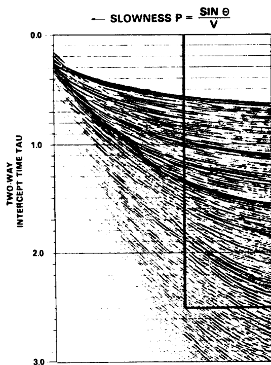
Figure 14: Gulf of Mexico data: Plane wave decomposition of a midpoint gather.
