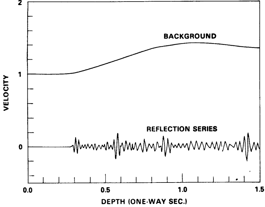
Figure 1: Background velocity and reflector series for synthetic examples.
