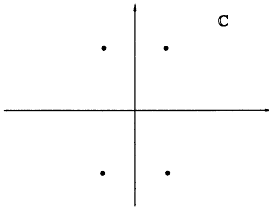
Figure 4.1: The case of an eigenvalue quadruplet.
