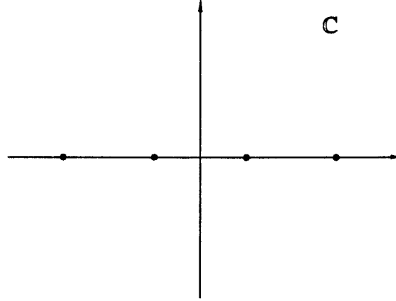
Figure 4.2: The case of eigenvalues on the real axis.
