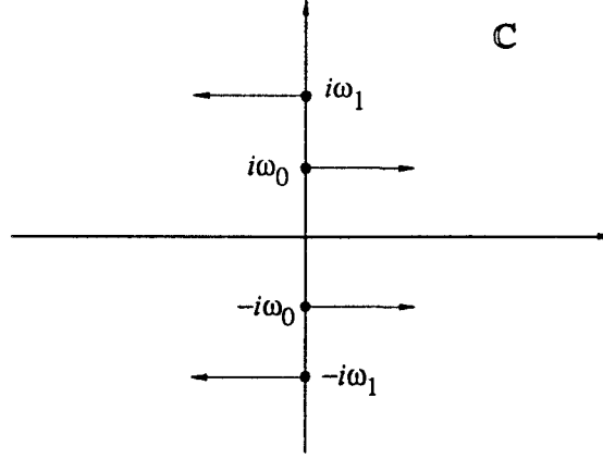
Figure 5.1: The weaker get destabilized.
