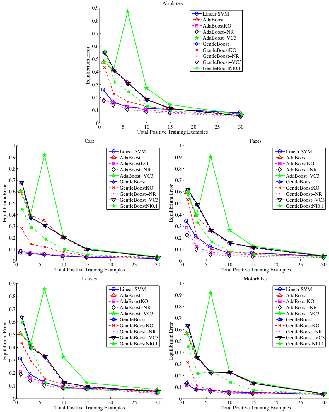
Figure B-1: A comparison between boosting variants using the C2 features on the five Caltech data sets: Airplanes, Cars, Faces, Leaves and Motorbikes. The graphs show the the equilibrium error rate vs. the number of training examples used from the class we want to detect. In each experiment, the test set was fixed to be the same as those described in [21], except for the random examples from the background set that were put aside for training. Each experiment was repeated 10 times.
