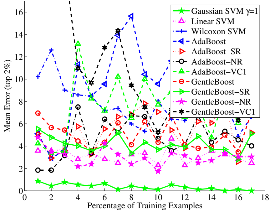
Figure 3-3: Classifier Performance on the HTD Data
