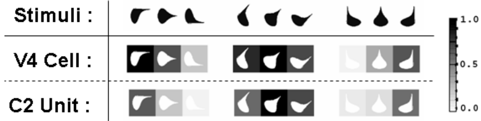
Figure 5: V4 cell and C2 unit response to the feature translation stimulus set. Responses are scaled between 0 and 1. V4 cell response is adapted from Figure 6B of [18].
