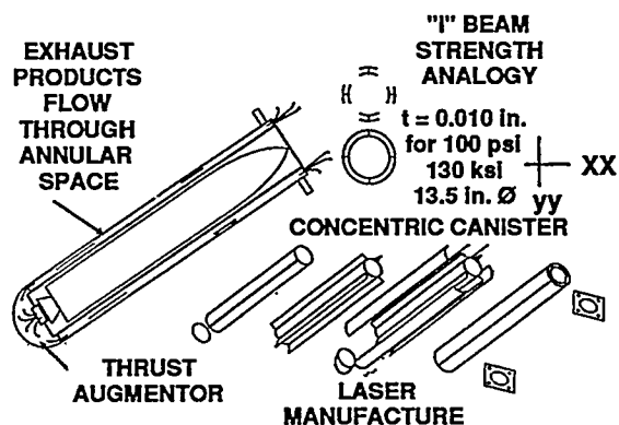
Figure 11. Concentric Canister Launcher approach
