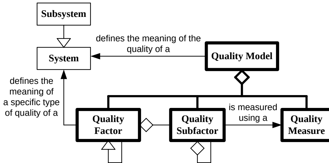
Figure 20: Quality Model
