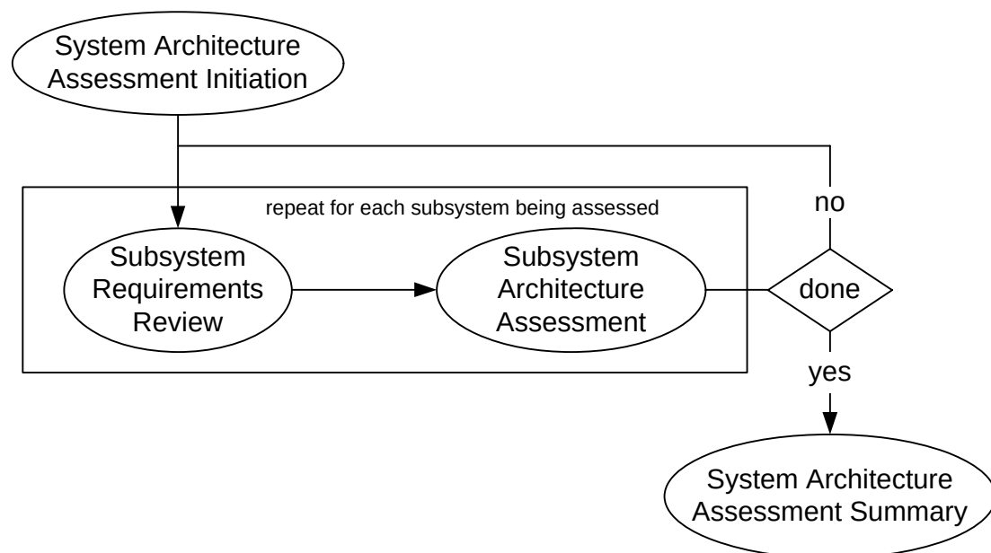
Figure 11: QUASAR Phases
