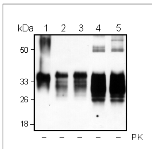
Figure 3. Immunoprecipitation of plasma PrP from normal and scrapie sheep. Except for PK treatment, refer to the legend in Fig. 2 for experimental protocol. As positive controls, approximately 1 ug of purified 263K/PrP Sc was processed using the same protocol as that used for plasma samples. Immune-complex captured on the beads were eluted with 2× SDS sample buffer and analyzed by 12% SDS-PAGE and Western blot using biotin-7A12. Lane 1: 263K brain homogenates as positive control for Western blot, lanes 2 & 3: plasma from normal and 263K-infected hamster, respectively, as positive controls for IP, lanes 4 & 5: plasma from normal and scrapie sheep, respectively.
