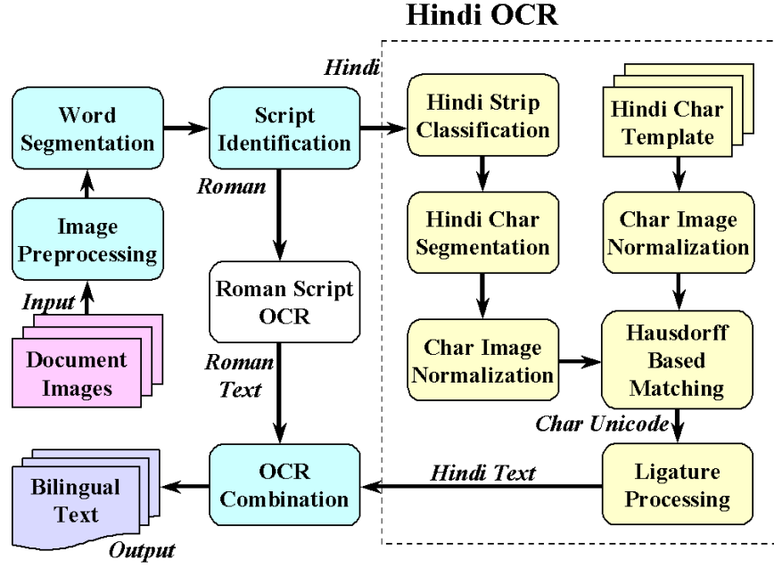
Figure 1: System architecture.
