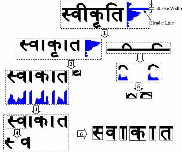
Figure 5: The procedure of Hindi character segmentation.
