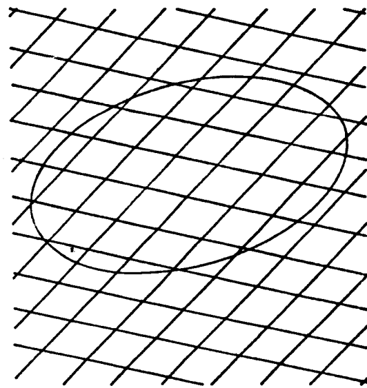
Fig. 4 A Rhomboidal grid in \mathbb{R}^2
