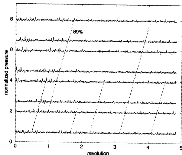
Figure 11 Pressure variation at 8 locations around annulus 90% chord ahead of the rotor of Stage 35 with injection
