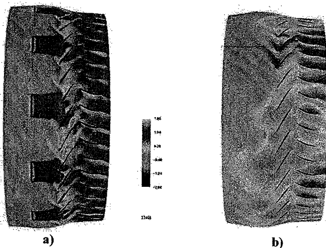
Figure 10 Axial velocity of Stage 35, a) with injection, and b) without injection
