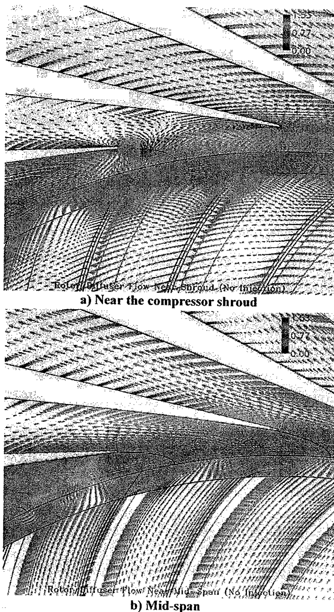
Figure 14 Blow up of instantaneous snap-shot of diffuser flow field at near stall condition, no injection.
