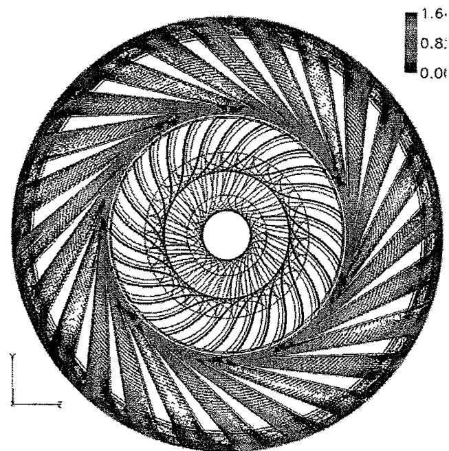
Figure 15 Diffuser flow field near shroud, with injection.
