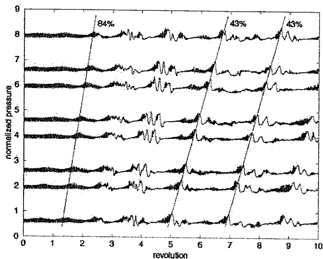
Figure 5 Time history of static pressure variation at 8 locations around the annulus located 90% chord ahead of the rotor of Stage 35 without injection.
