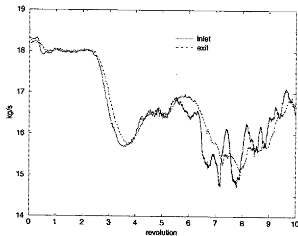
Figure 6 Mass flow variation during stall inception process of Stage 35.
