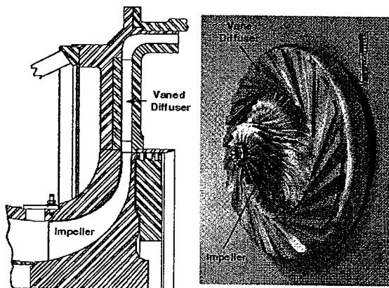
Figure 2 High-speed centrifugal compressor, CC3, validation case.
