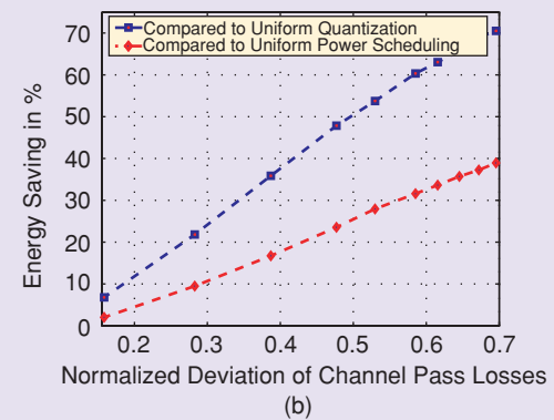
[FIG9] (a) Number of active sensors decreases as the channel path losses become more heterogeneous. (b) Power savings compared to uniform power scheduling or uniform quantization.
