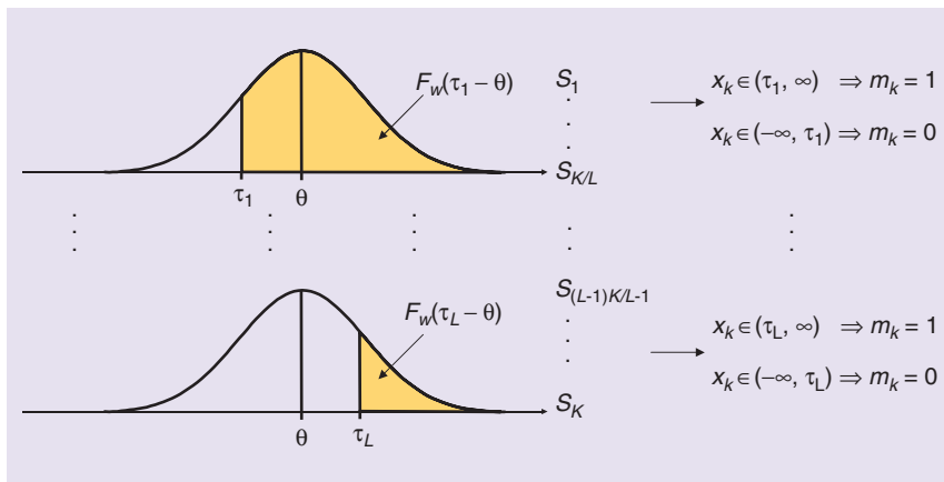
[FIG5] When the noise pdf p_w(w; \psi) is known but depends on L unknown parameters we divide the sensors in L groups each using a different threshold \tau_l to construct the binary message m_k . Note that the messages are Bernoulli distributed with parameters q_l := \Pr\{x_k \in (\tau_l, \infty)\} = F_w(\tau_l - \theta) when sensor S_k uses the threshold \tau_l .
