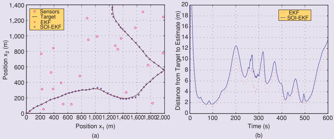
[FIG10] Target tracking with EKF and SOI-EKF.
