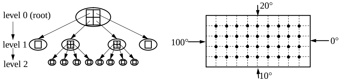
Figure 8. On the left is a tree of Stencil instances. In this case a 4-ary tree. On the right is the canonical grid approximation of a heated plate used in our PDE example.
