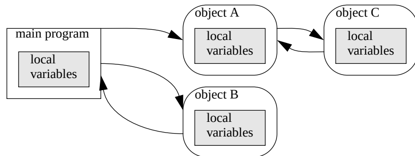
Figure 1 The Mentat object model. Mentat objects are address space disjoint and communicate via member functions and return values, shown here as directed arcs. Both the main program and Mentat objects may contain local variables.
