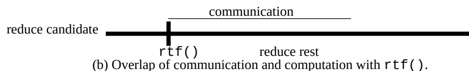
Figure 2 Gaussian elimination with partial pivoting illustrating the use of rtf()
