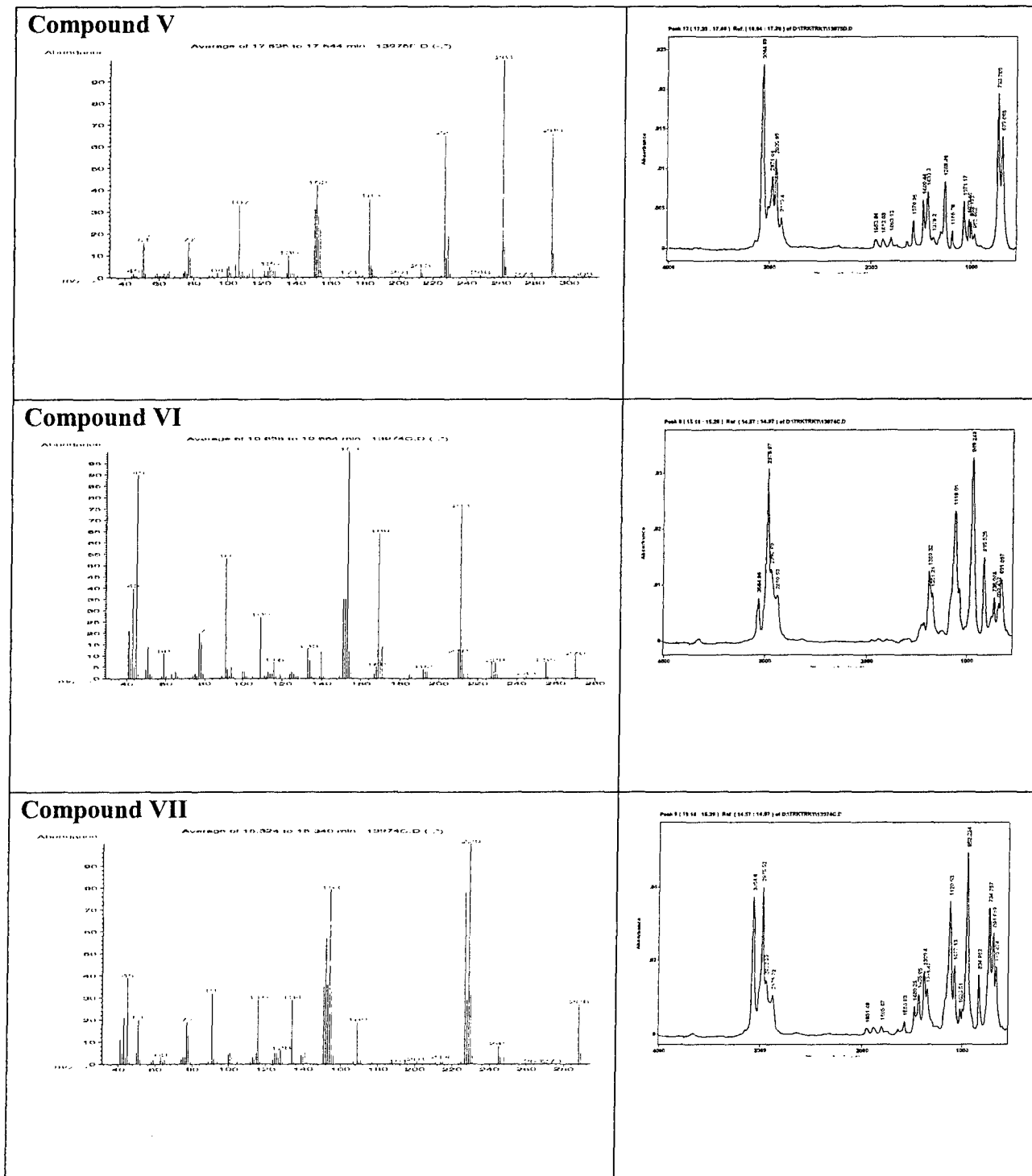
Figure 16. Mass and Infrared Spectra of Chemicals Identified During the Gas Chromatographic Analyses.
