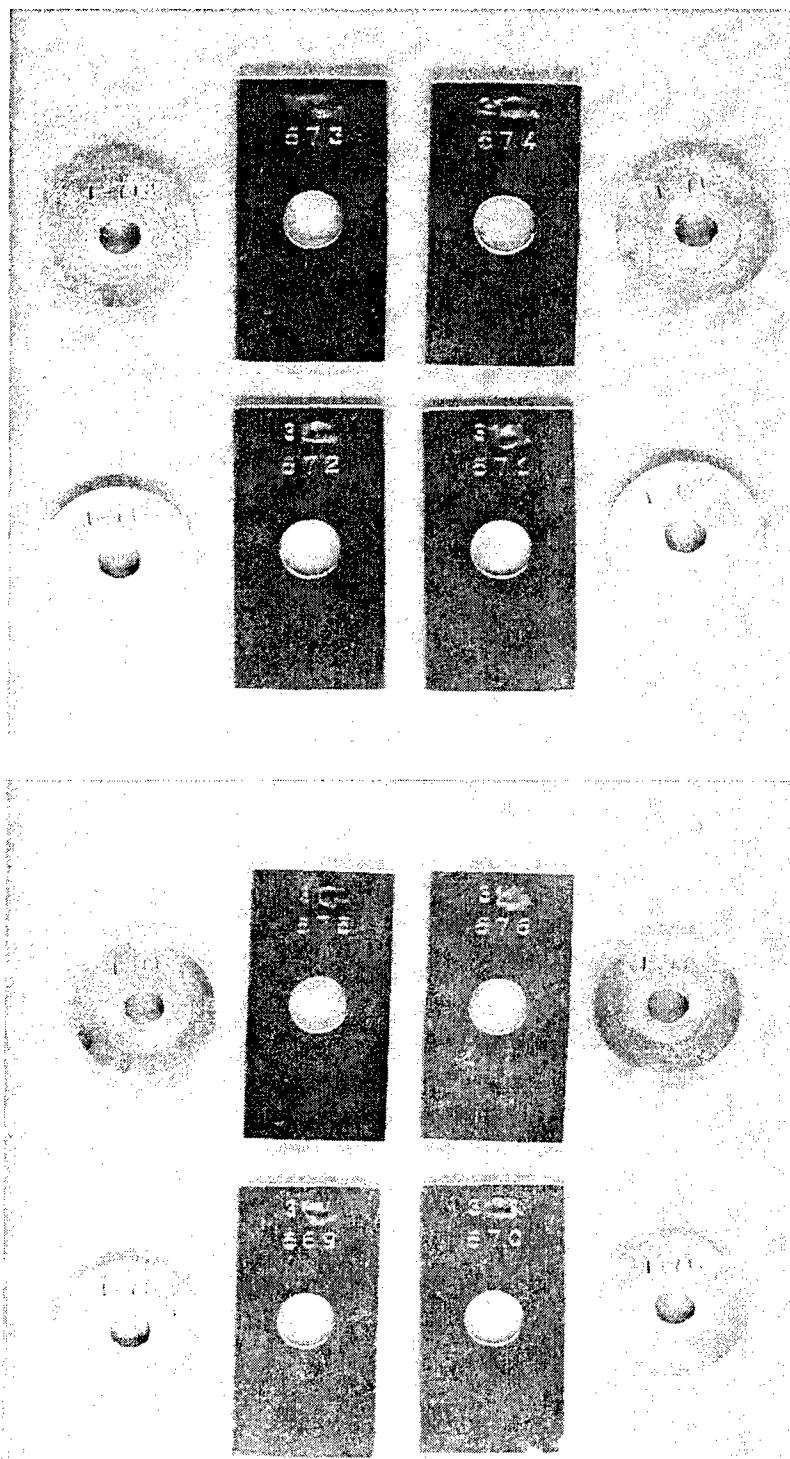
Figure 71. Metal Specimens with Galvanic-Crevice Assemblies Exposed to Arsinol/Permanganate Neutralent for 120 hr. The top panel is the 60 °C exposure, and the bottom panel is the 80 °C exposure. In each panel, the top specimens were partially immersed, and the bottom specimens were fully immersed.
