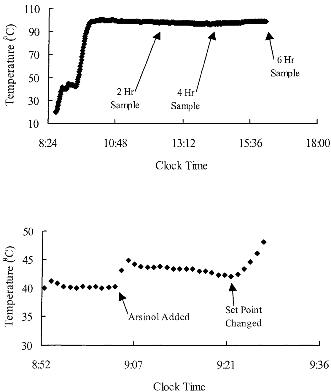
Figure 38. Temperature Profile for the 1:25 Loading Reactor Run, with a Final Temperature of 100 °C. The upper panel is full-scale, and the lower panel is zoomed into the arsinol addition time-frame.
